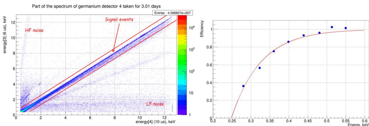
Figure 6. Left: Example of the Fourier analysis made with different shaping times. Right: survival fraction of the events from pulse generator after applying all the cuts
