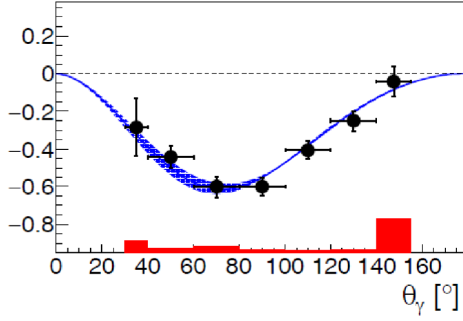
Figure 9: Beam asymmetry \Sigma_3 in the range 119-139 MeV. Points – experiment, the curve – ChPT calculation (publication [1]).
