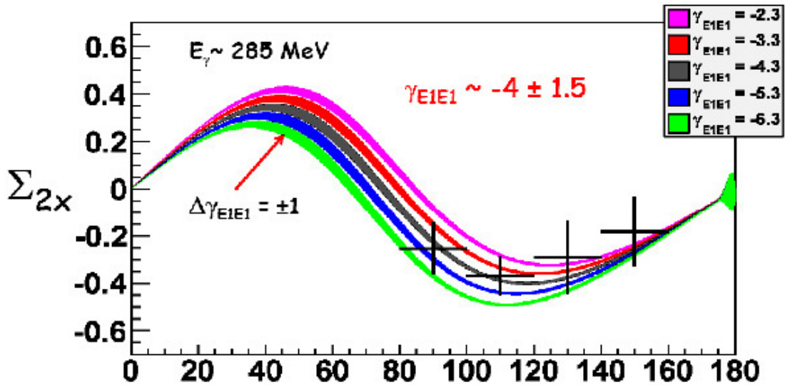
Figure 8: Proton spin polarizability \gamma E1E1 obtained from the measurement of the Compton scattering asymmetry \Sigma 2x . The points are the experimental data, the curves are dispersion model calculations. The horizontal axis indicates the scattering angle.
