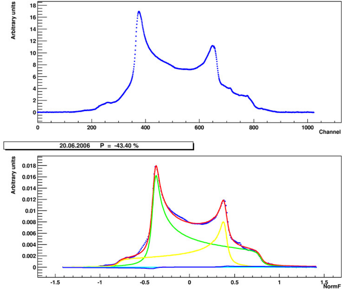
Figure 13: Absorption DMR spectra with the maximum achieved polarization are presented. Top plot: experimental spectrum. Bottom plot: points – experimental spectrum; the components correspond to: 0 \longleftrightarrow -1 transition (green line), 1 \longleftrightarrow 0 transition (yellow line), whole DMR spectrum (blue line), sum of the decomposition of a spectrum on the components (red line).
