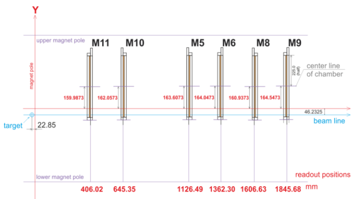
Positions of half-planes for the RUN-7 configuration
