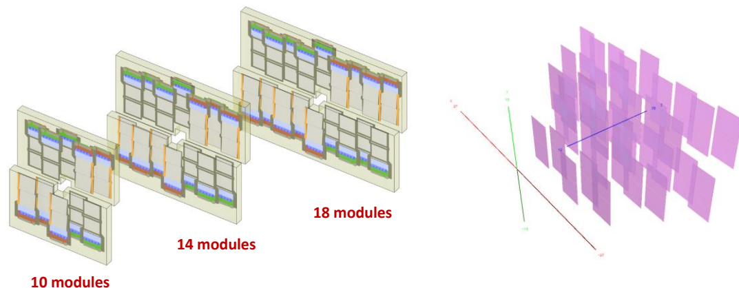
Three stations of the Forward Si detector (left) and ROOT geometry of them for MC-simulation (right)
