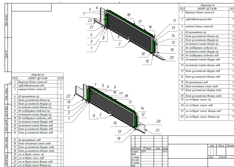
Drawing of two GEM half-planes (upper and lower) for the future runs
