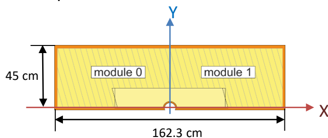
GEM half-plane with sizes of 163x45 cm
