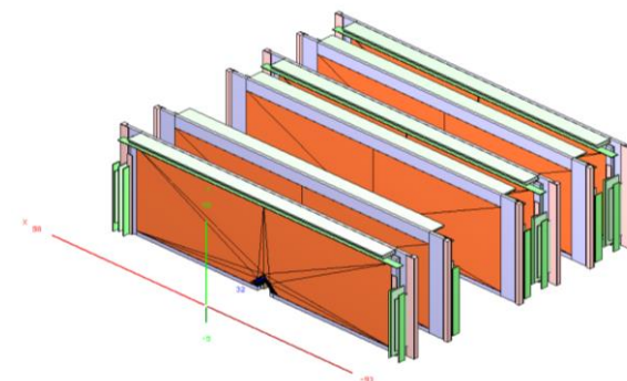
Detailed ROOT geometry of GEMs for RUN-7: passive elements (such as frames, electronics and material layers in sensitive areas) were added.
