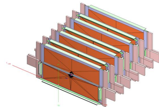
Detailed ROOT geometry of GEMs for the next run: passive elements (such as frames, electronics and material layers in sensitive areas) were added.
