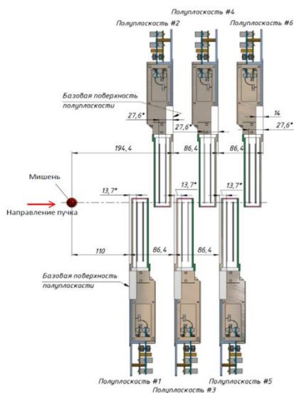
Scheme of the Forward Si detector
