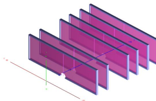
Simplified ROOT geometry of GEMs for RUN-7: only sensitive planes (as volumes filled with a gas mixture) and ordinary frames.
