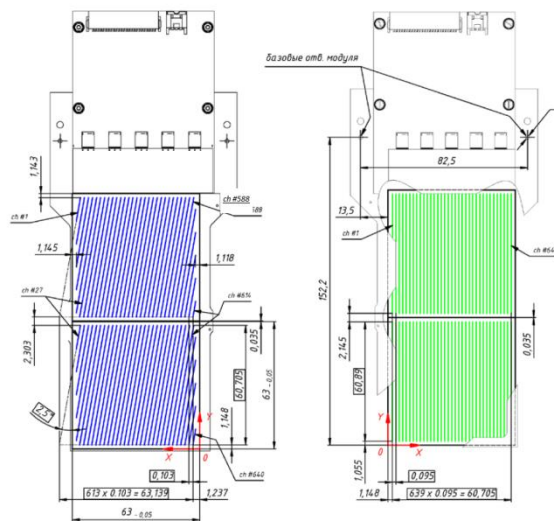
Schemes of a single Si-module (left) and their composition in the first station (right)
