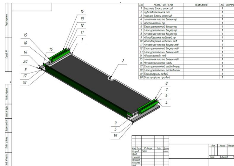
One drawing of the GEM half-plane
