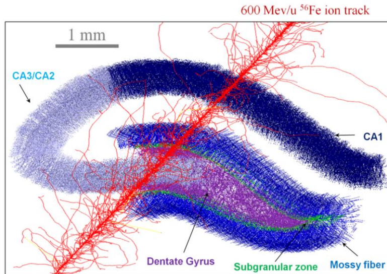
Fig. A Monte Carlo simulation of a 600 MeV/n 56 Fe ion track structure in a three-dimensional model of the rat hippocampus including main zones and cell types indicated by different colours.
