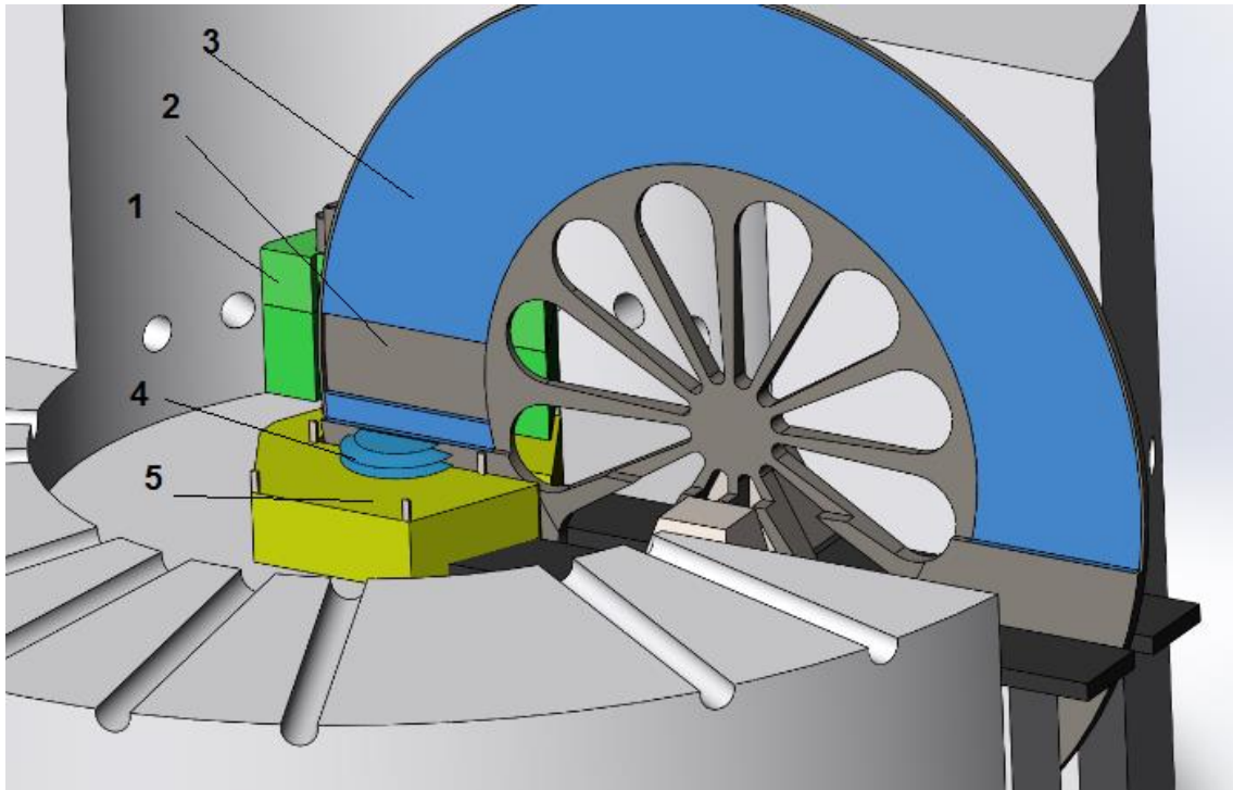
Figure : schematic view of the IBR-3: 1- reactor core reactor core, 2 - empty sector of reactivity modulator, 3 - reactivity modulator coated with titanium hydride coating, 4 - moderator, 5 - beryllium reflector.
