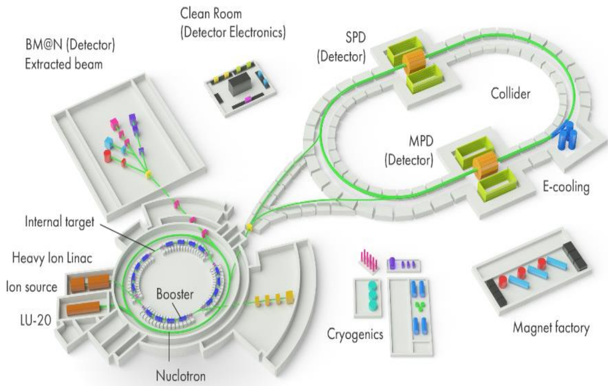
Figure: The NICA accelerator complex
