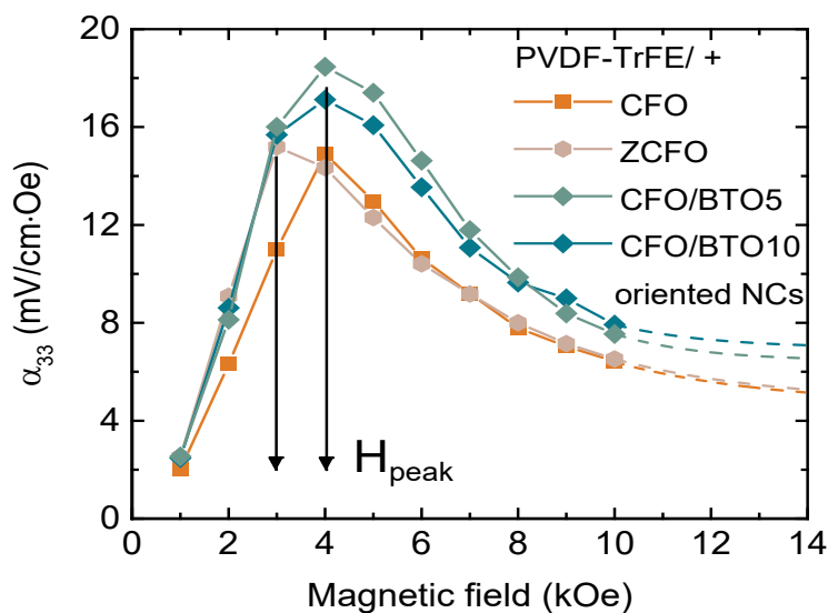
Fig. 1. Dependencies of the ME voltage coefficient ( \alpha_{ME} ) on DC bias magnetic field composites at AC field frequency of 10 kHz for PVDF-TrFE -based samples with ZCFO, BTO5/CFO and BTO10/CFO fillers.
