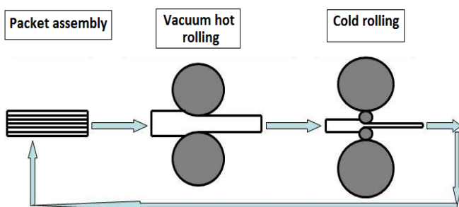
Fig. 1. Obtaining multilayer composites. Scheme of one cycle.
