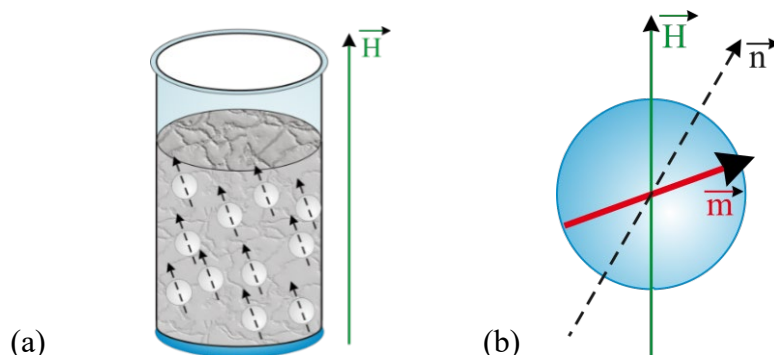
Figure 1. Sketche of the sample studied: (a) immobilized randomly distributed superparamagnetic particles with perfect alignment of the magnetic easy axes in some direction; (b) model of a superparamagnetic nanoparticle. The orientation of the particle is given by the body-fixed, magnetic easy axis vector \mathbf{n} . The orientation of the particle magnetic moment \mathbf{m} can be different from the easy-axis vector due to superparamagnetic fluctuations.
