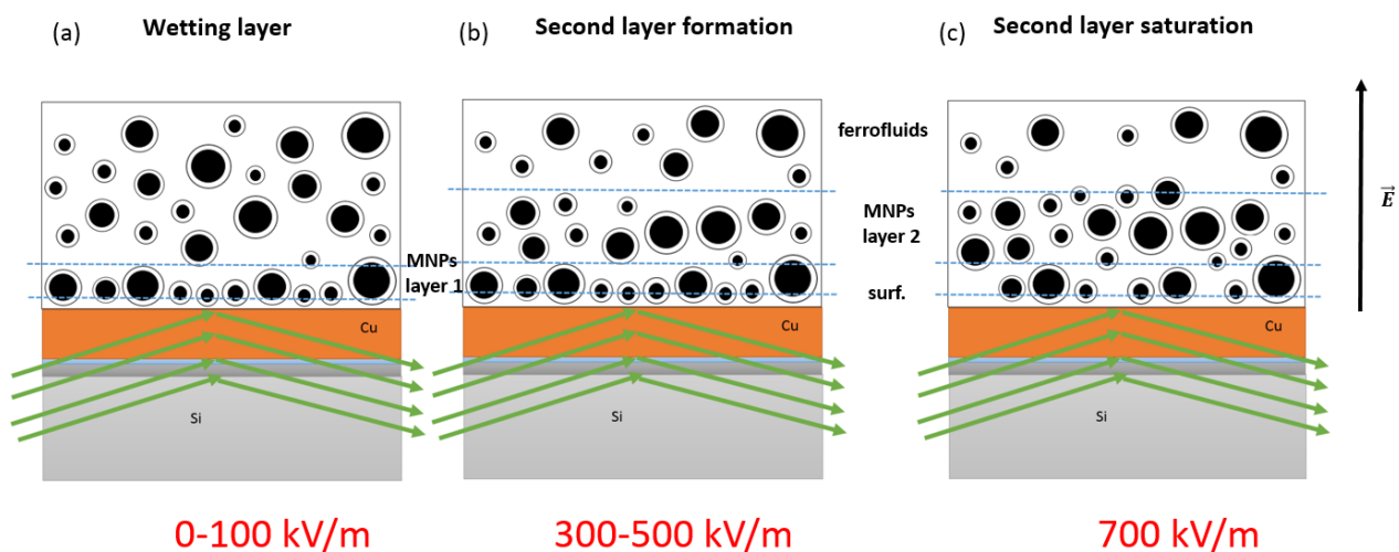
Fig. 1. Schematic drawing of NP-ordering determined from the results of neutron reflectometry: (a) wetting layer; (b) double layer on top of the wetting layer in an electric field 300-500 kV/m; (c) saturated double layer on top of the wetting layer in an electric field of 700 kV/m.
