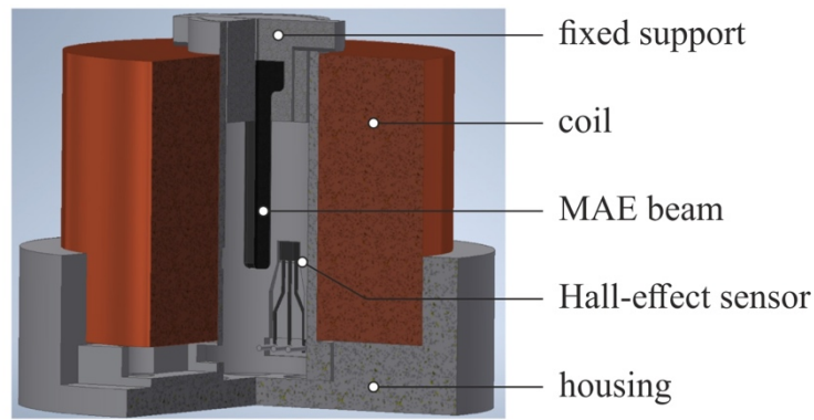
Figure 1. Prototype of an MAE-based vibrating sensor element
