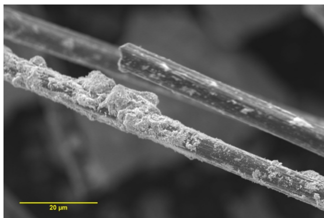
Fig. 1. SEM-image of modified CF by magnetite particles
