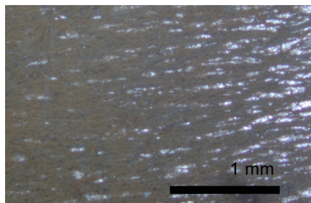
Fig. 1 Film structure of a magnetic elastomer
