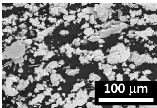
Fig.1. Image of the aggregates of the permalloy particles.
