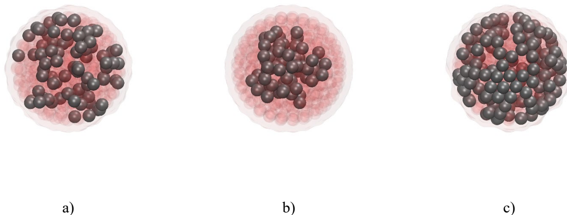
Figure 1. Initial MNPs distributions in microgel sample: a) randomly filled, b) magnetic core – polymeric shell, c) polymeric core – magnetic shell.
