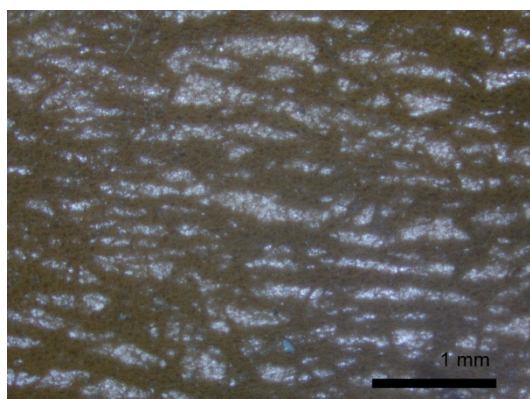
Fig. 1 Film structure of a magnetic elastomer
