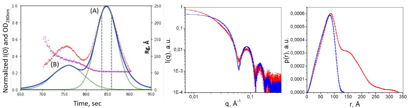
Figure 1. SEC-SAXS profile of apoferritin (Left), I(q) and p(r) dependencies (Middle and Right, respectively) corresponding to peak fractions (A) (blue curves) and (B) (red curves).
