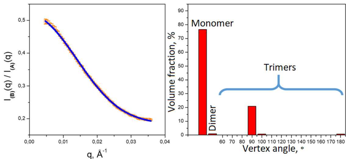
Figure 2. Experimental intensity ratio I(B)(q)/I(A)(q) (orange points) and corresponding fit (blue curve) (Left) and histogram of volume fractions of apoferritin monomers, dimers and trimers (Right).
