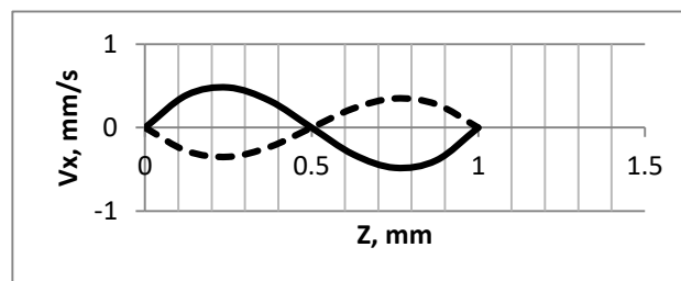
Figure 1 - The longitudinal component of the velocity v_x with respect to the z coordinate at a fixed x = 10 mm. Dotted line: time t = 0.5 s; solid: t = 1 s. The angular frequency of the field is \omega \sim 10 rad/s; volume concentration of particles in the center of the cloud \Phi_0 = 0.01 ; gap thickness l = 1 mm.
