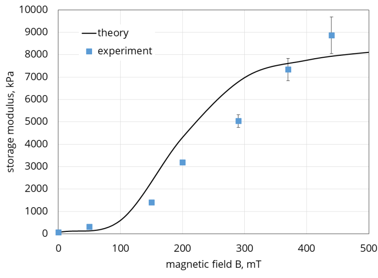
Figure2. Shear modulus vs. the applied magnetic field.. Volume concentration of the embedded particles is 30%. Modulus of the sample without the field is 10 kPa.
