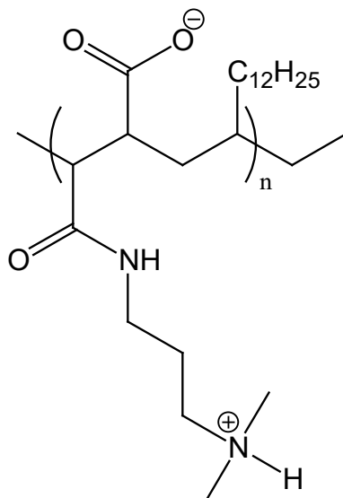
Figure 2. The chemical structure of amphiphilic polymer PMAL-C12
