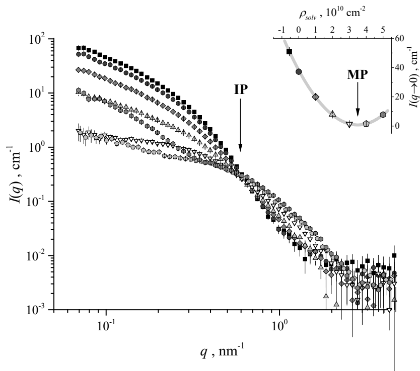
Figure 1. Changes in experimental SANS curves with contrast variation for \text{Fe}_3\text{O}_4\text{-}2\cdot\text{DBSA-H}_2\text{O} magnetic fluid. Curves are plotted with the same color and point style as the corresponding points in inset, where the change in the forward scattering intensities with varying solvent SLD is shown. Arrows indicate isoscattering point (IP) as well as effective match point (MP) corresponding to the minimum of quadratic dependency (solid line).
