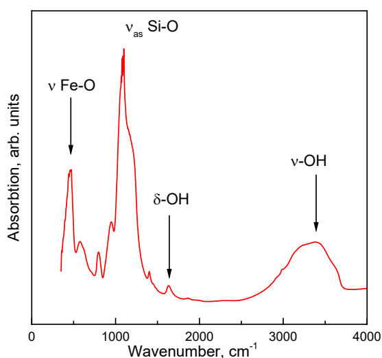
Fig.1. Room-temperature FTIR spectrum of \text{Fe}_3\text{O}_4@\text{SiO}_2
