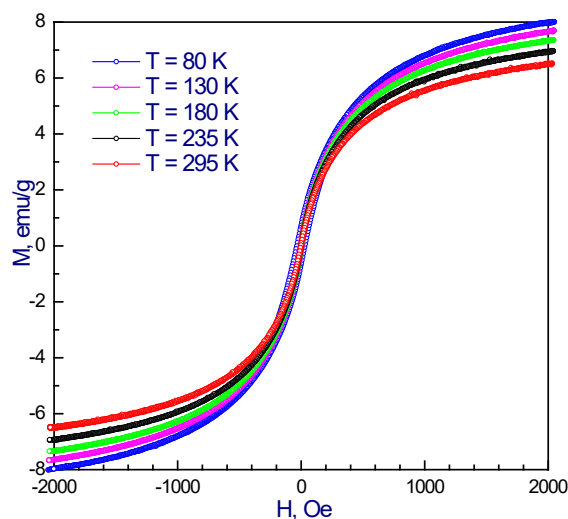
Fig.2. Hysteresis loops
