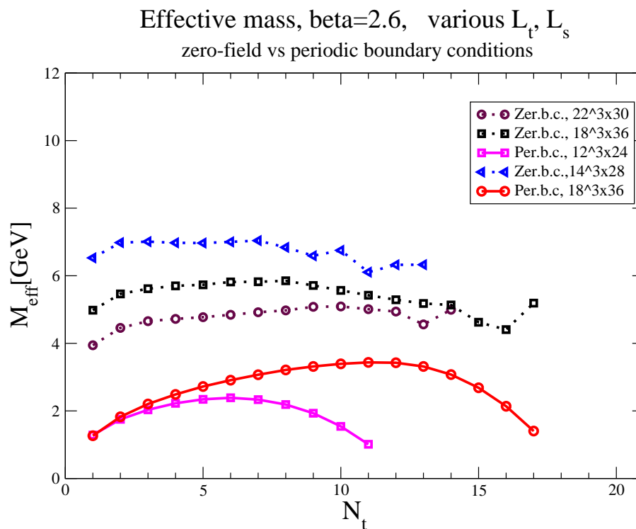
Figure 5: Comparison of effective masses m(t) for zero-field and periodic BCs, for various L_s and L_t at \beta = 2.6 .
