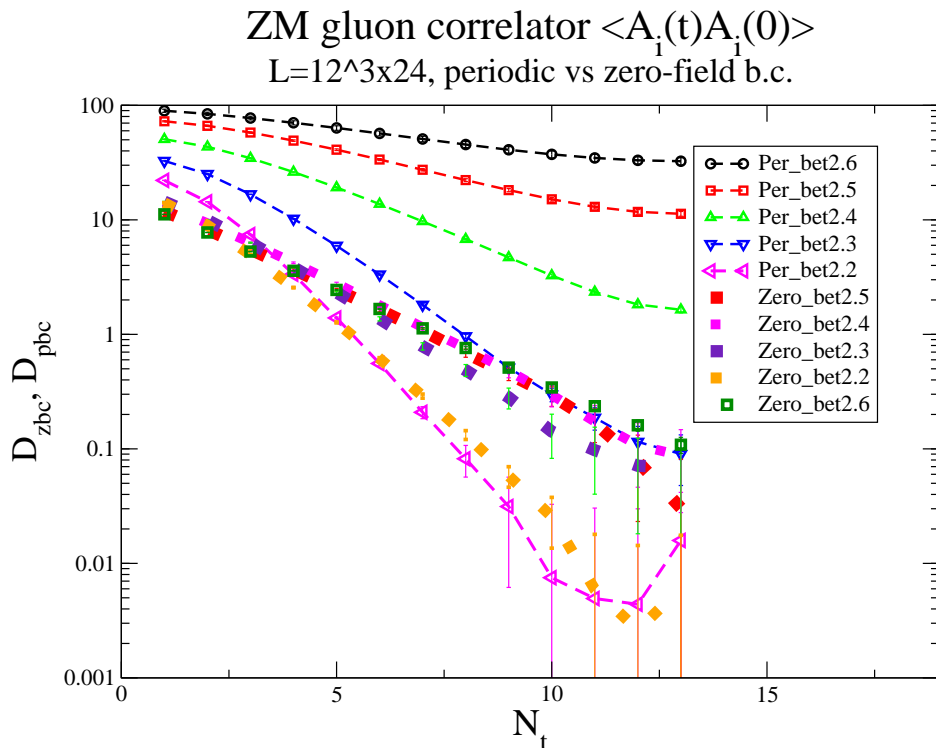
Figure 4: Comparison of the ZM gluon correlator S(t) for zero-field and periodic BCs, L_s = 12 and various \beta .
