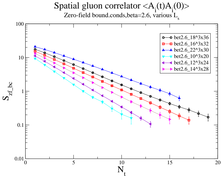
Figure 3: The ZM gluon propagator S(t) for \beta = 2.6 , ZF BCs and various lattice sizes .
