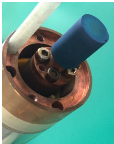
Figure 2. Installation of the cold cathode.
