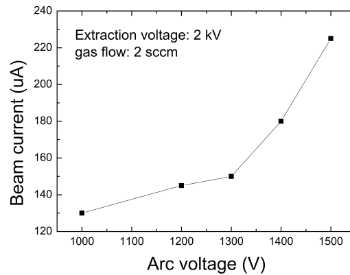
Figure 9. Extracted beam current vs. arc voltage.
