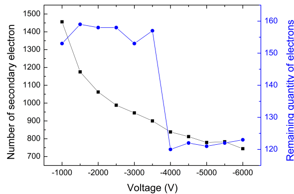
Figure 5. The results of secondary electron simulation.
