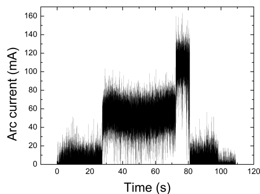
Figure 8. Arc current waveform under 1400V arc voltage.
