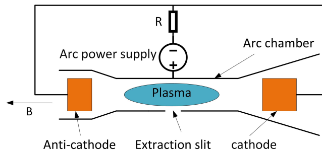
Figure 1. Structure diagram of cold cathode ion source.
