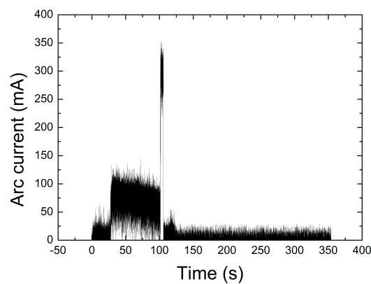
Figure 7. Arc current waveform under 1500V arc voltage.
