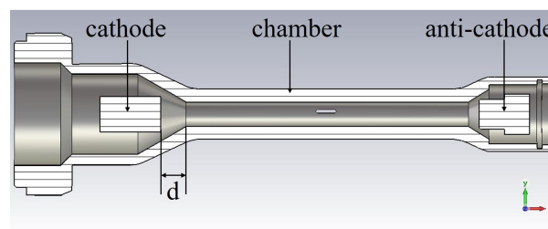
Figure 3. Cold cathode ion source model for simulation.
