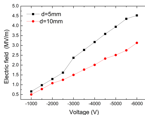
Figure 4. Cathode surface electric field vs. voltage applied to the cathode.
