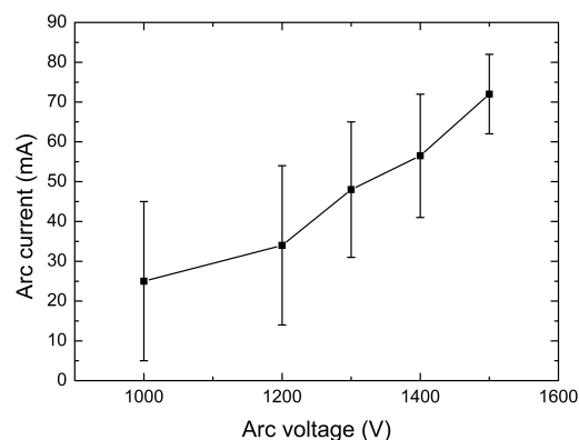
Figure 6. Arc current vs. arc voltage.
