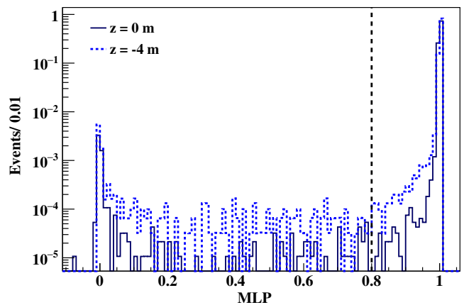
FIG. 29. Distribution of the MLP \alpha/\beta discriminator (Sec. III D) for the gammas from the capture of neutrons from ^{241}\text{Am} - ^9\text{Be} calibration source placed at the detector center (x, y, z) = (0, 0, 0) m, as well as at (0, 0, -4) m, where the observed distribution is the broadest. The dashed line shows the threshold set at 0.8 for the delayed in IBD search.
