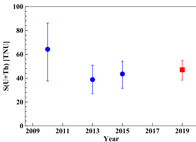
FIG. 51. Comparison of the geoneutrino signal S_{\text{geo}}(U + \text{Th}) at LNGS as measured by Borexino. Blue circles indicate the results from 2010 [16], 2013 [17], and 2015 [18], while the red square demonstrates the current analysis.
