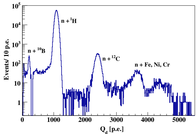
FIG. 13. The N_{pe} charge spectrum of delayed signals, expressed in the number of detected photoelectrons, due to the gammas from captures of neutrons emitted from the ^{241}\text{Am}-^9\text{Be} calibration source placed in the center of the detector. The clearly visible peaks of 2.22 MeV and 4.95 MeV gammas from the neutron captures on proton and ^{12}\text{C} are positioned at 1090 p.e. and 2400 p.e., respectively. The other peaks are from neutron captures on nuclei of stainless steel used in the source and its insertion system construction: at >7 MeV energies due to captures on (Fe, Ni, Cr) and at 477.6 keV on ^{10}\text{B} .
