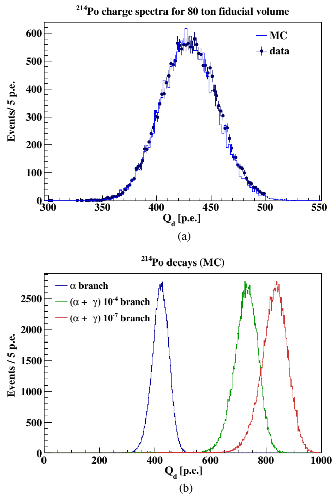
FIG. 41. Top: Comparison of the charge spectra of \alpha decays from ^{214}\text{Po} from data (circles with error bars) and MC (solid line) in the fiducial volume of \sim 80 tons around the detector center chosen to tune the alpha particle quenching factor. Bottom: Charge distributions for the three ^{214}\text{Po} decays (Table XI) obtained using MC with the \alpha energy scale tuned on pure \alpha -decays [Fig. 41(a)]. The main \alpha decay (red line) and the two subdominant (\alpha + \gamma) branches are shown: 10^{-4} (green line) and 10^{-7} (blue line) branch. The three spectra are normalized to have the same area.
