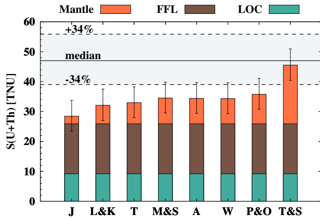
FIG. 50. Comparison of the expected geoneutrino signal S_{\text{geo}}(U + \text{Th}) at LNGS (calculated according to different BSE models, see Sec. VB) with the Borexino measurement. For each model, the LOC and FFL contributions are the same (Table VI), while the mantle signal is obtained considering an intermediate scenario [Fig. 16(b)]. The error bars represent the 1\sigma uncertainties of the total signal S(U + \text{Th}) . The horizontal solid back line represents the geoneutrino signal S_{\text{geo}}^{\text{med}} , while the grey band the I_{S_{\text{geo}}}^{68\text{full}} interval as measured by Borexino.
