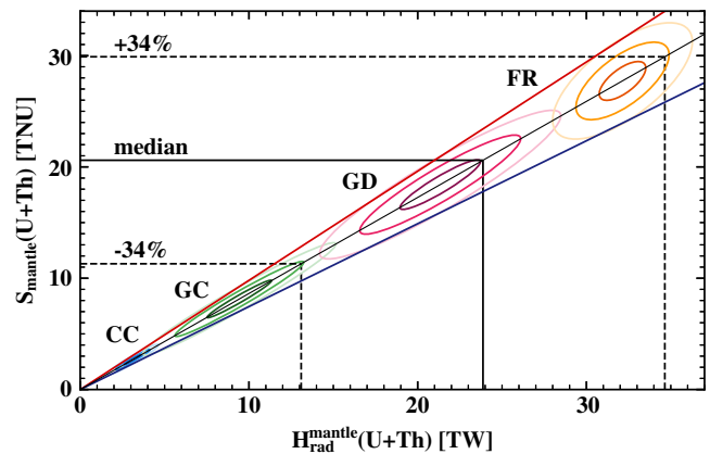
FIG. 54. Mantle geoneutrino signal expected in Borexino as a function of U and Th mantle radiogenic heat: the area between the red and blue lines denotes the full range allowed between a homogeneous mantle [high scenario—Fig. 16(c)] and a unique rich layer just above the CMB [low scenario—Fig. 16(a)]. The slope of the central inclined black line ( \beta_{\text{centr}} = 0.86 TNU/TW) is the average of the slopes of the blue and red lines. The blue, green, red, and yellow ellipses are calculated with the following U and Th mantle radiogenic power H_{\text{rad}}^{\text{mantle}}(\text{U} + \text{Th}) (with 1\sigma error) according to different BSE models: CC model ( 3.1 \pm 0.5 ) TW, GC model ( 9.5 \pm 1.9 ) TW, GD model ( 21.3 \pm 2.4 ) TW, and FR model ( 32.2 \pm 1.4 ) TW. For each model darker to lighter shades of respective colors represent 1, 2, and 3\sigma contours. The black horizontal lines represent the mantle signal measured by Borexino: the median mantle signal (solid line) and the 68% coverage interval (dashed lines).
