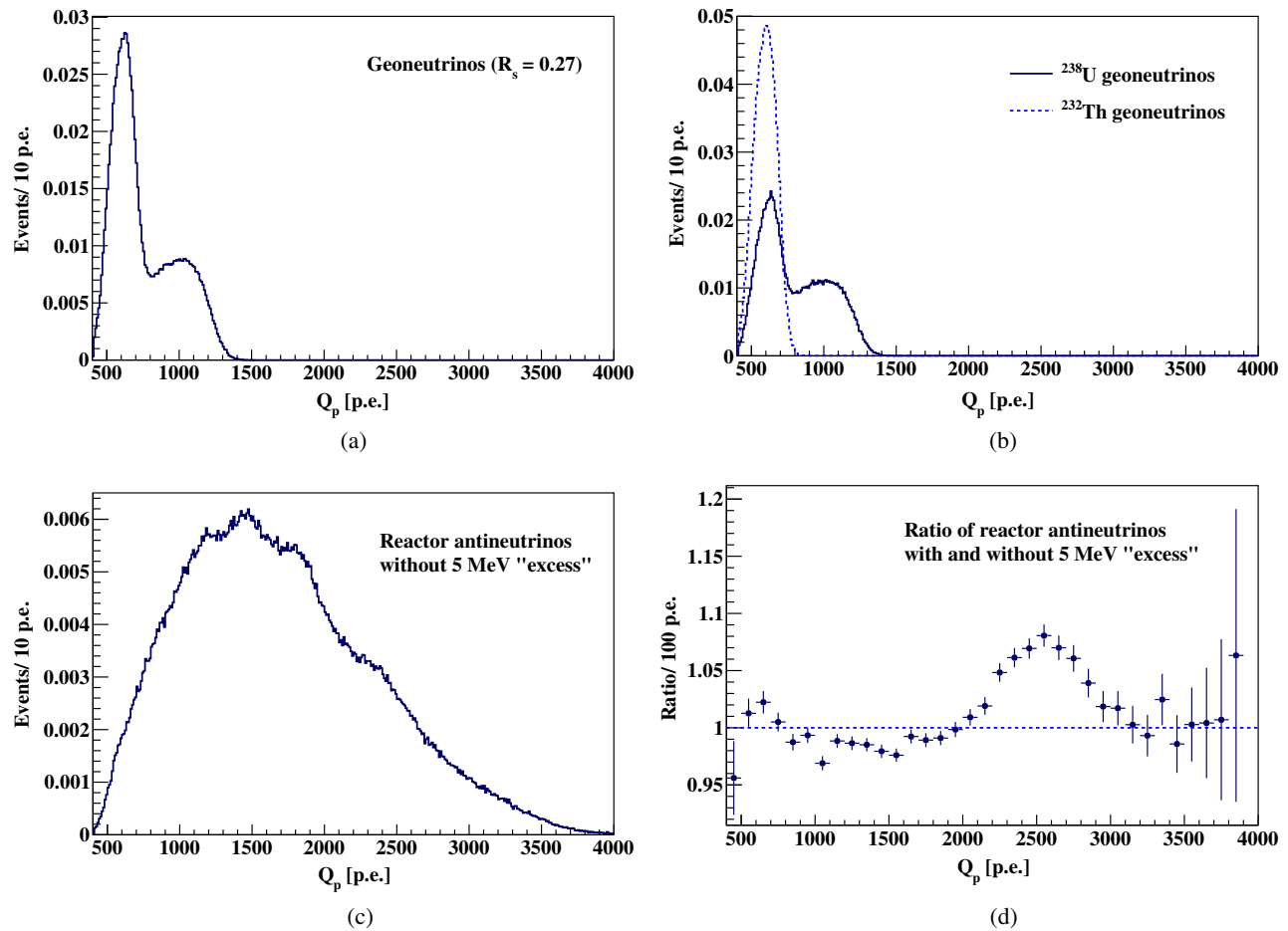
FIG. 32. The MC-based PDFs normalized to one, i.e., the expected shapes of prompts for geoneutrinos and reactor antineutrinos, after optimized geoneutrino selection cuts, that include the detector response. Top-left: geoneutrinos with Th/U ratio fixed to the chondritic value ( R_S = 0.27 ). Top-right: ^{238}\text{U} and ^{232}\text{Th} PDFs shown separately. Bottom-left: reactor antineutrinos “without 5 MeV “excess.”” Bottom-right: ratio of reactor antineutrino spectra “with/without 5 MeV “excess”” (Sec. V C), normalized to the same number of events each, in order to demonstrate the difference in shape only.
