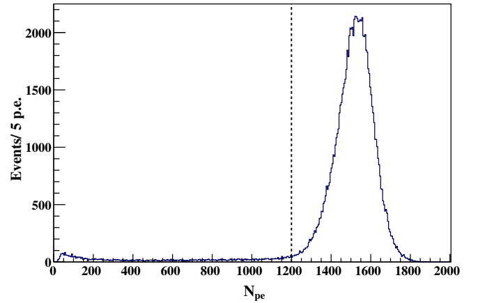
FIG. 39. The N_{pe} distribution of 3 MeV \gamma s generated in the DFM and in the entire analyzed period of geoneutrino analysis. The vertical line indicates the 1200 p.e. threshold used in the evaluation of the (\gamma, n) background.
