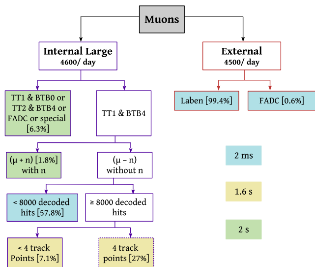
FIG. 23. Scheme of different types of vetoes applied after various muon categories. The relative fraction of each muon category is given by the numbers in brackets. Different colors represent different durations of the time veto. The dashed line around the box at the bottom of the plot represents the only muon category when the cylindrical veto around the muon track is applied. For other categories, the whole detector is vetoed.
