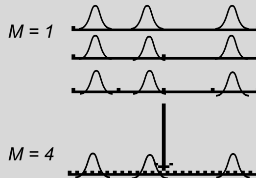
Nonpoint-like groups with width \sigma
