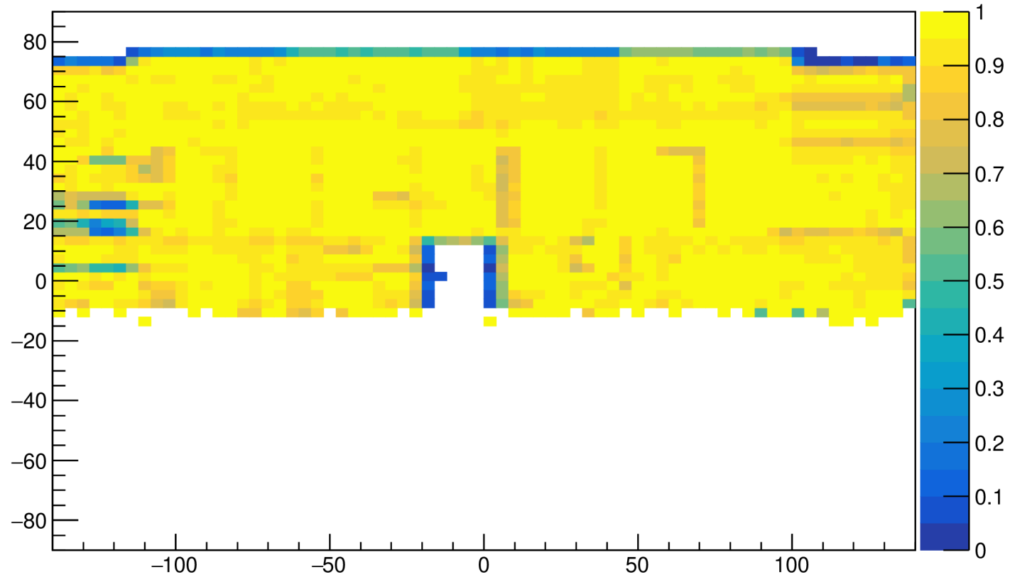
Efficiency GEM+DCH+TOF700 vs XY good GEM+DCH tracks
