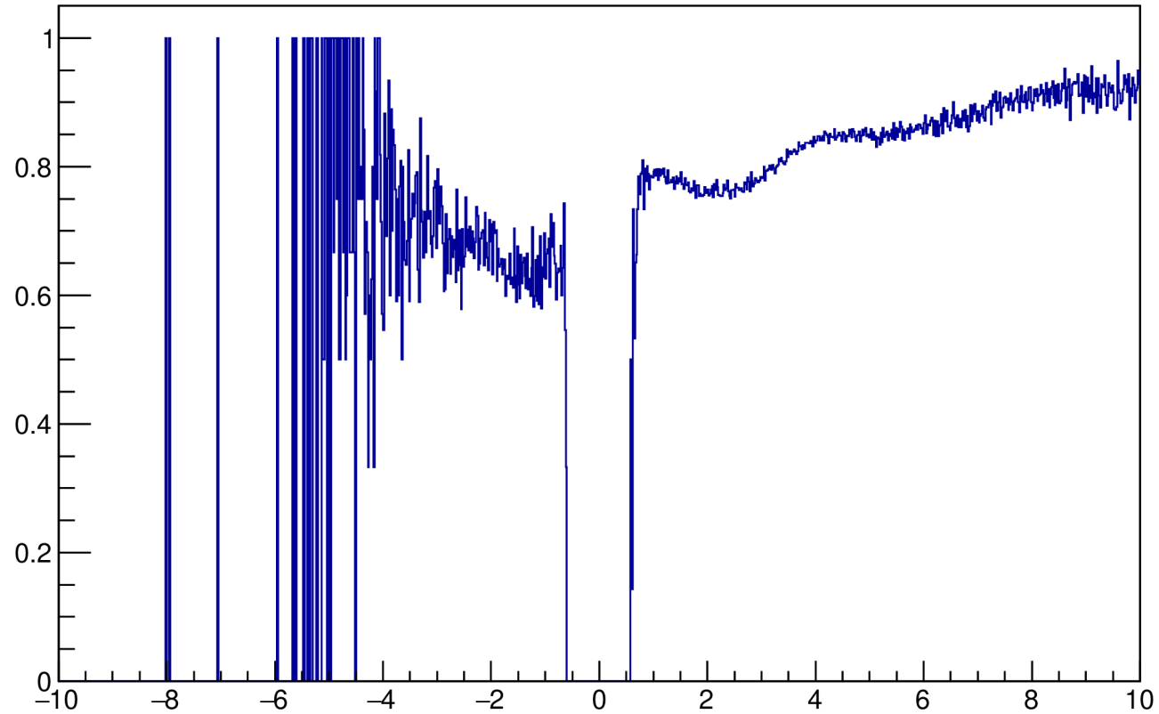
Efficiency GEM+DCH+TOF700 vs P good GEM+DCH tracks
