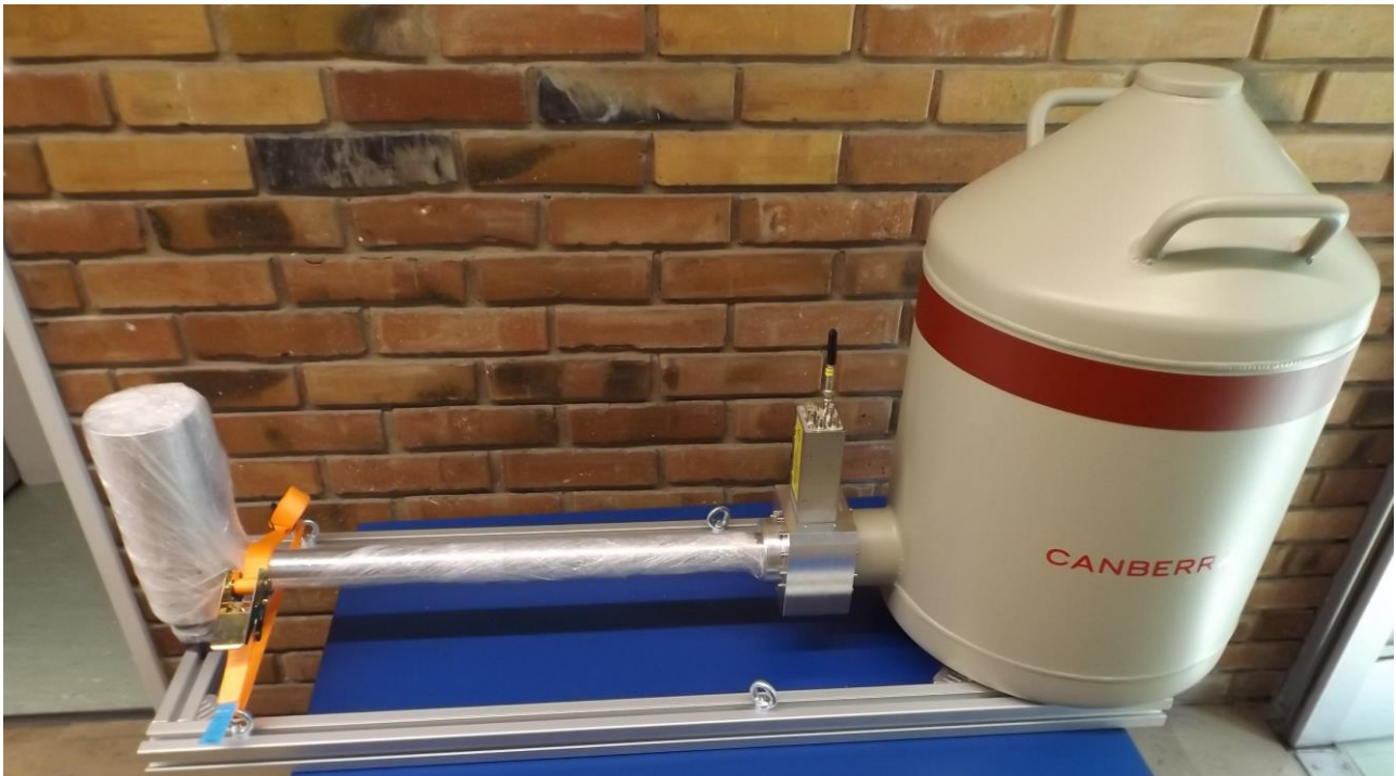
Figure 2. Photo of one HPGe point contact vGeN detectors.
