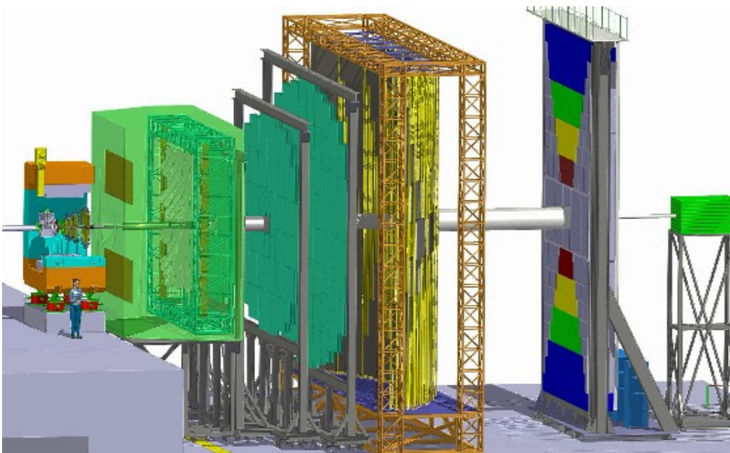
Figure 3: CBM setup for electron detection option. It includes superconducting dipole magnet, Vertex Detector, Silicon Tracker System, Ring Imaging Cherenkov detector, Transition Radiation Detector, Time of Flight System based on Resistive Plate Chambers, Electromagnetic Calorimeter, Projectile Spectator Detector.
