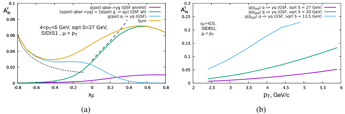
Figure 2.13: (a) x_F -dependence of the asymmetry A_N^\gamma calculated based on the SIDIS1 Siverts function for \sqrt{s} = 27 GeV and 4 < p_T < 6 GeV/c. Gluon and quark contributions are shown separately by color solid lines. Dashed lines illustrate the twist-3 predictions for \sqrt{s} = 30 GeV and p_T = 4 GeV/c for negative [145] and positive [131] values of x_F . (b) p_T -dependence of the A_N^\gamma asymmetry for different values of \sqrt{s} at x_F = -0.5 .
