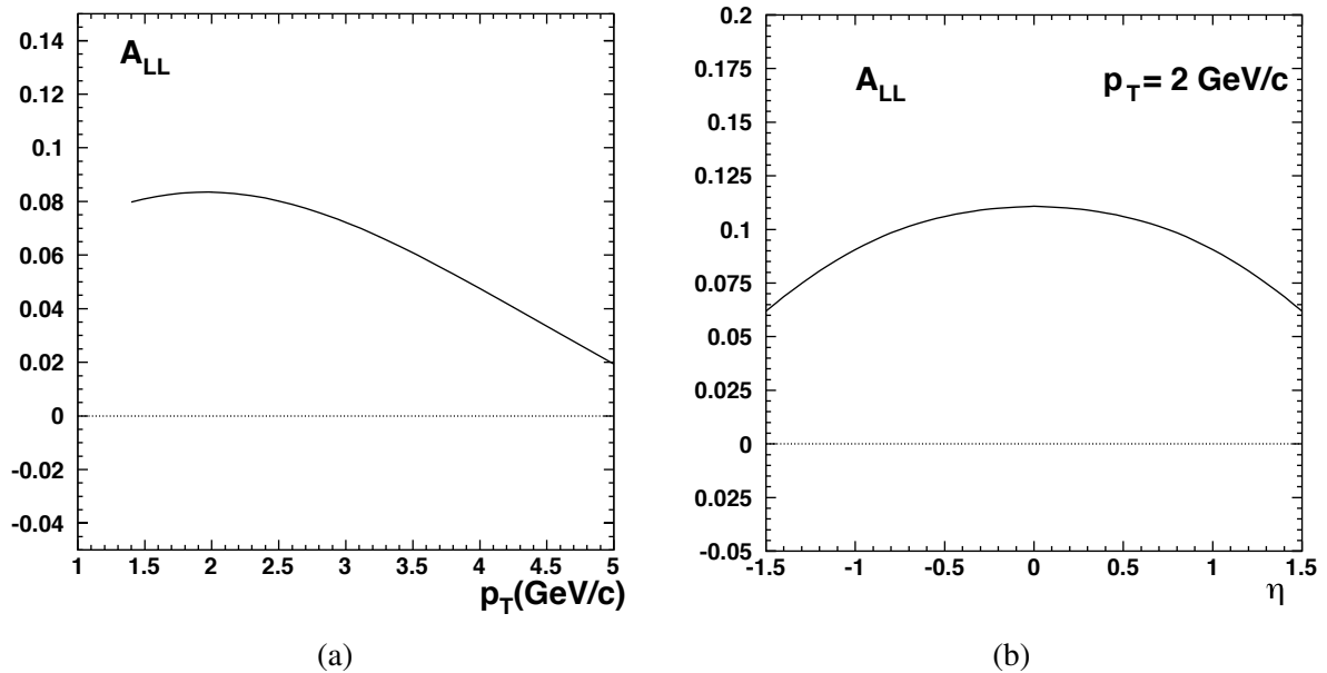
Figure 2.8: Longitudinal double spin asymmetry A_{LL} for inclusive J/\psi production calculated for p - p collisions at \sqrt{s} = 39 \text{ GeV} in the LO approximation as a function of a) transverse momentum p_T and b) pseudorapidity \eta [122].
