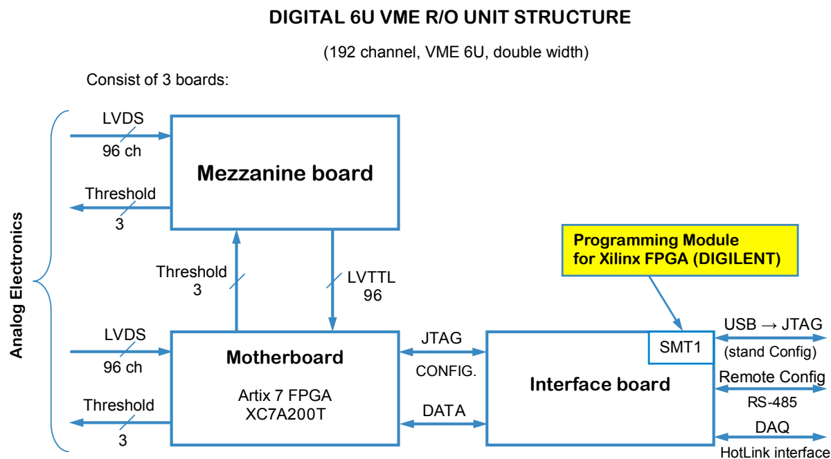
Figure 4.31: Block-diagram of the MFDM module.
