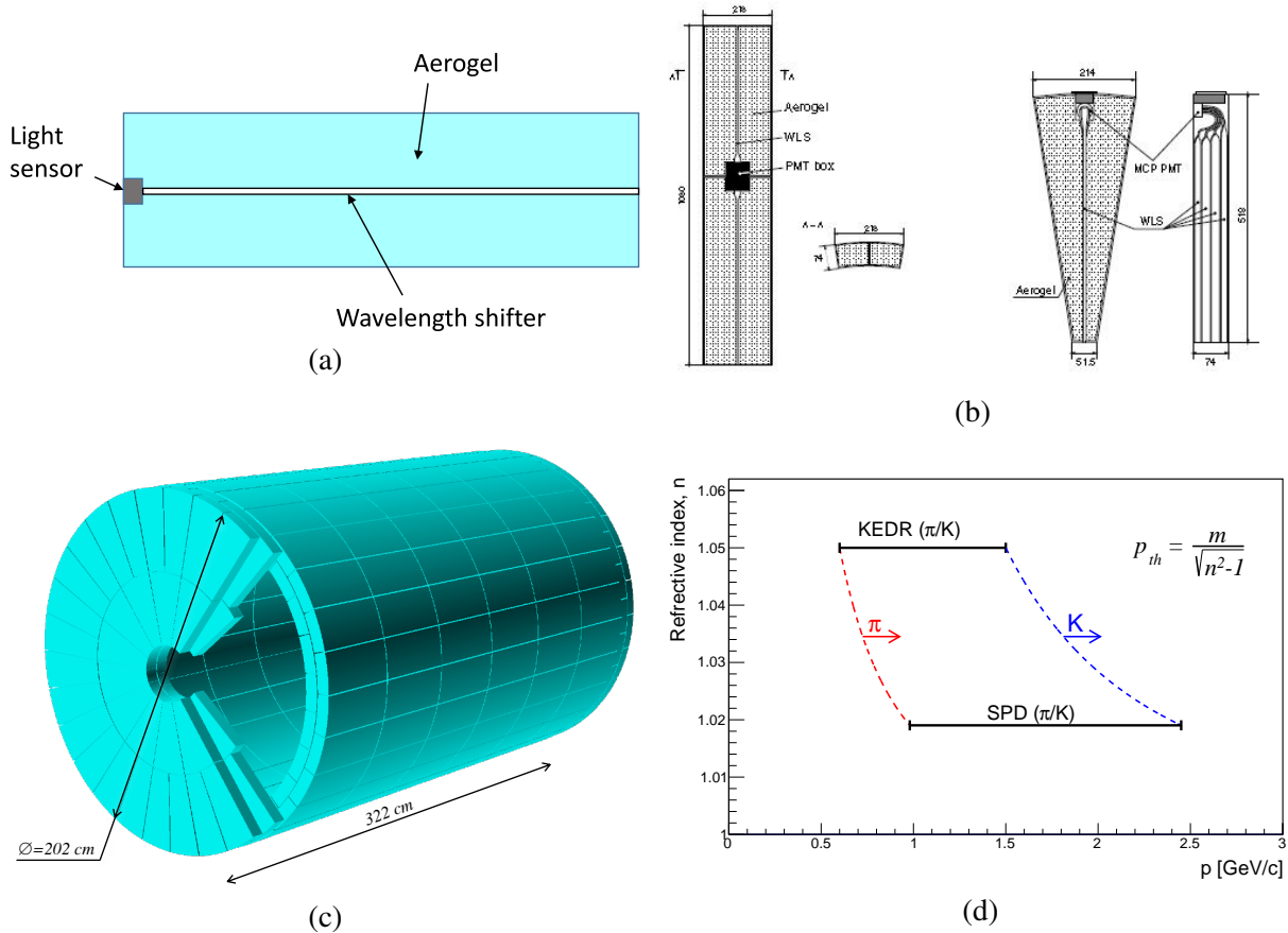
Figure 4.38: (a) Principle of ASHIPH operation. (b) KEDR aerogel counters: two barrel counters in a single housing (left), end-cap counter (right) [408]. (c) Possible arrangement of barrel and end-cap counters in SPD. (d) Momentum intervals of KEDR and SPD where the \pi/K separation is possible.
