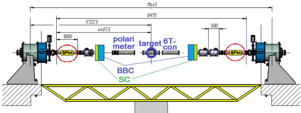
Figure 11.2: The SPD straight section equipped with the diagnostic and control units. All dimensions are in millimeters.
