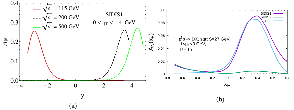
Figure 2.11: (a) Predictions for A_N^{J/\psi} for \sqrt{s} = 115 GeV (AFTER), 200 GeV and 500 GeV (RHIC) as a function of rapidity y [140]. (b) Siverts effect contribution to the A_N^D asymmetry calculated within the Generalized Parton Model.
