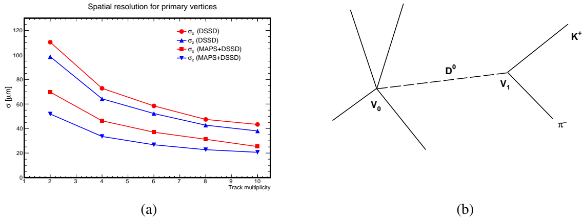
Figure 9.6: (a) Accuracy of the primary vertex position reconstruction as a function of the number of outgoing tracks for two configurations of the vertex detector. (b) Sketch of D^0 -meson production and decay.
