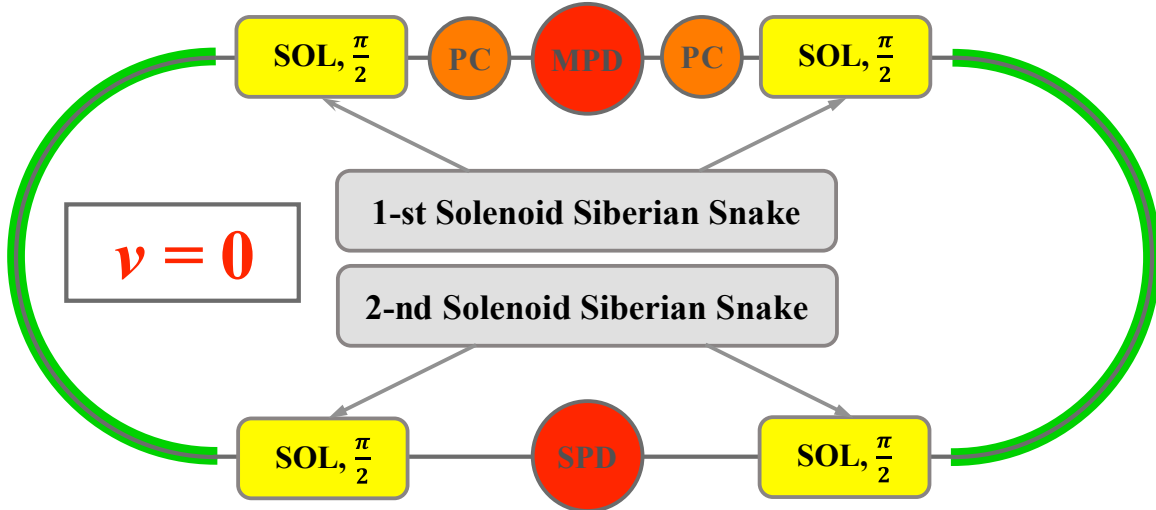
Figure 3.6: Implementation of the ST regime in the NICA collider.
