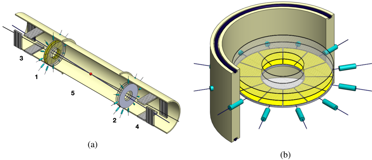
Figure 4.40: (a) Possible layout: the Fast Beam-Beam Collision (FBBC [412]) monitor composed of MCP discs (1 and 2) in combination with the Beam Position devices (BPM) (3 and 4) are situated symmetrically to the Interaction Point (5) inside the vacuum beam pipe of the NICA collider. (b) Compact module of the Fast Beam-Beam Collision Monitor (FBBC) based on circular MCPs. Sector cathode readout pads and two MCP setups are embedded into a separate flange with a hermetic 50- \Omega signal and HV feedthroughs (the latter are not shown).
