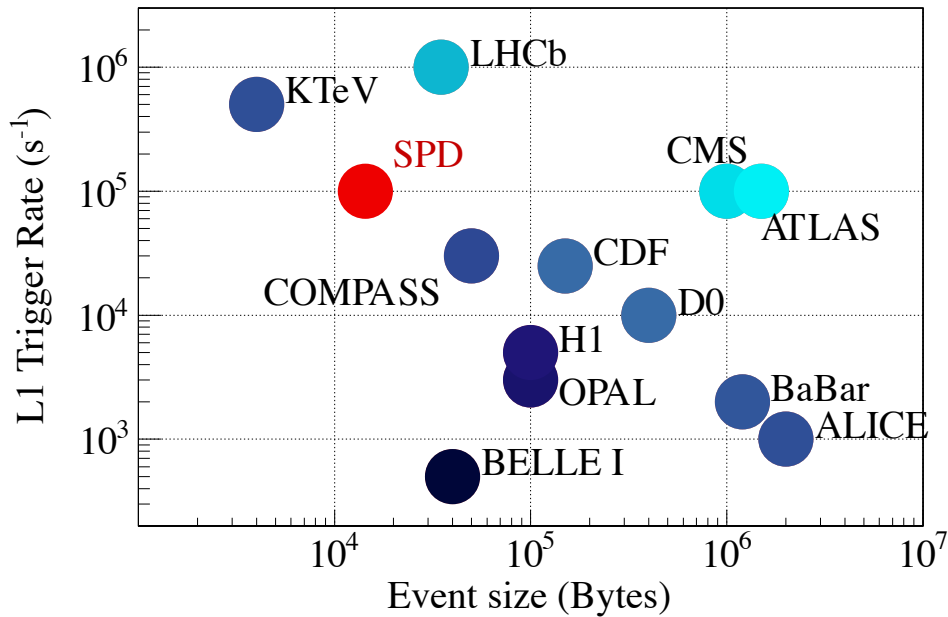
Figure 8.1: Expected event size and event rate of the SPD setup after the online filter compared with other experiments [445].
