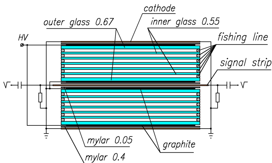
Figure 4.36: Schematic view of the twelve-gap mRPC [397].
