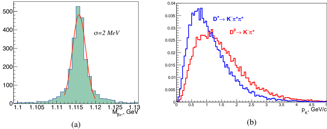
Figure 9.8: (a) \Lambda peak in the p\pi mass spectrum. (b) Kaon spectra from the decays D^0 \rightarrow K^- \pi^+ (red) and D^+ \rightarrow K^- \pi^+ \pi^+ (blue) produced at \sqrt{s} = 27 \text{ GeV}/c .
