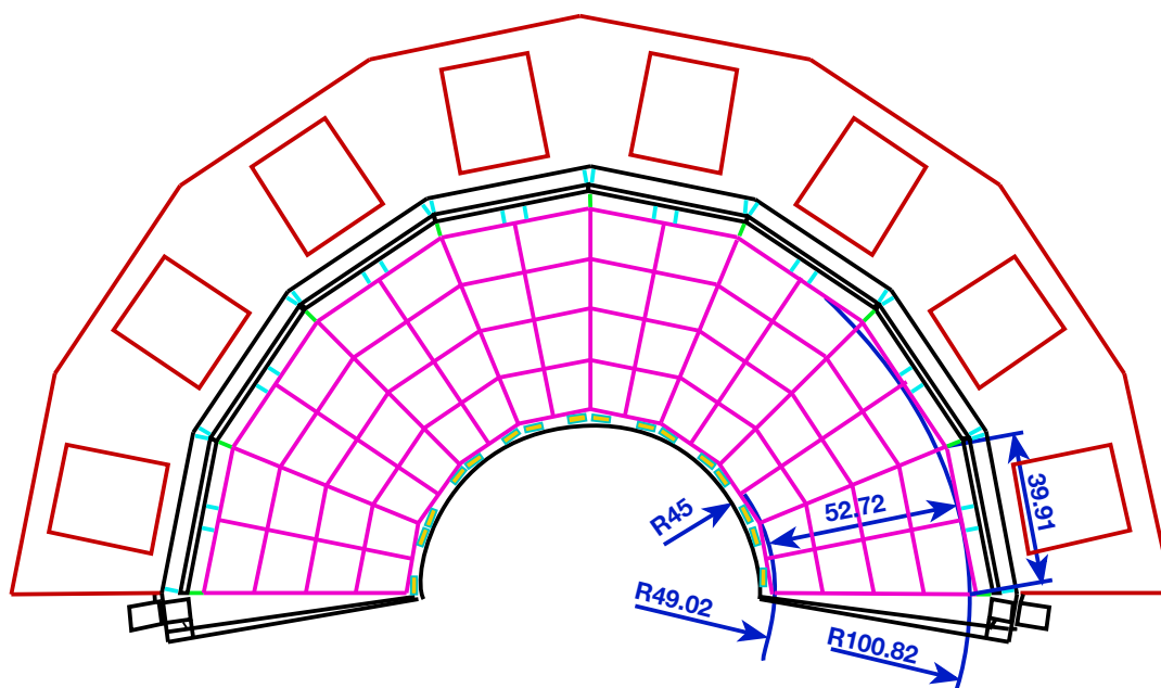
Figure 4.39: Beam-Beam Counter: azimuthal and polar angle segmentation [411]. All dimensions are in millimeters.
