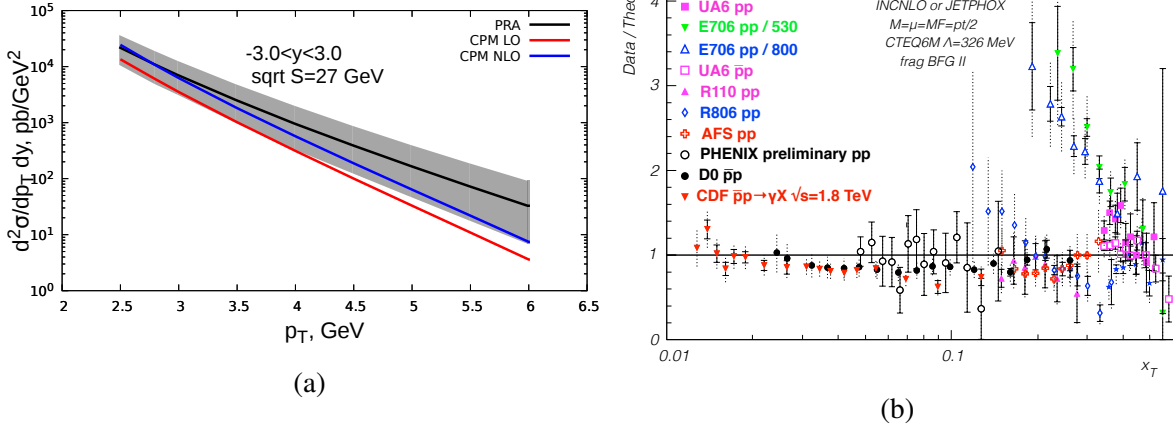
Figure 2.3: (a) Prediction for prompt photon transverse momentum spectrum at \sqrt{s} = 27 GeV obtained in LO (red line) and NLO (blue line) approximations of CPM and LO of PRA (black line). Uncertainty bands for PRA predictions are due to factorization/renormalization scale variation only. (b) Data-to-theory ratio for the fixed-target and collider experiments [33].
