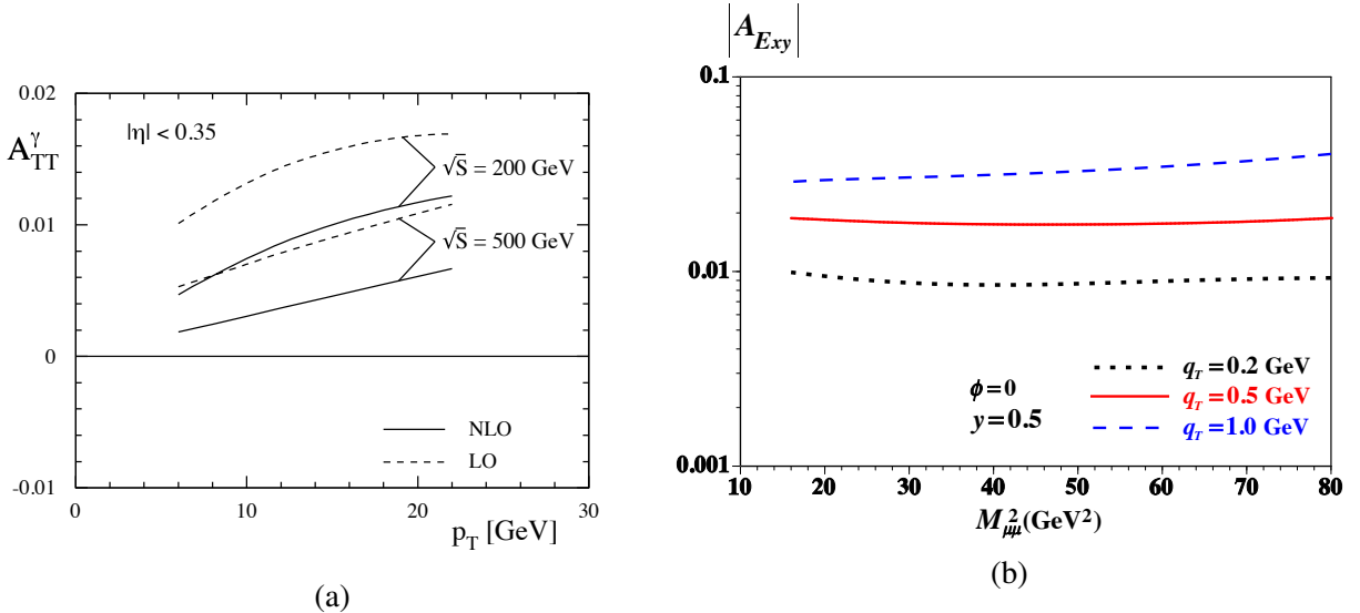
Figure 2.14: (a) A_{TT}^\gamma asymmetry for the prompt-photon production at 200 and 500 GeV coming from the q\bar{q} annihilation process calculated in LO [152] and NLO [153]. (b) Spin asymmetries |A_{E_{xy}}| for the proton-deuteron Drell-Yan process as a function of the dimuon mass squared for the dimuon rapidity y = 0.5 and different transverse momenta q_T [151].
