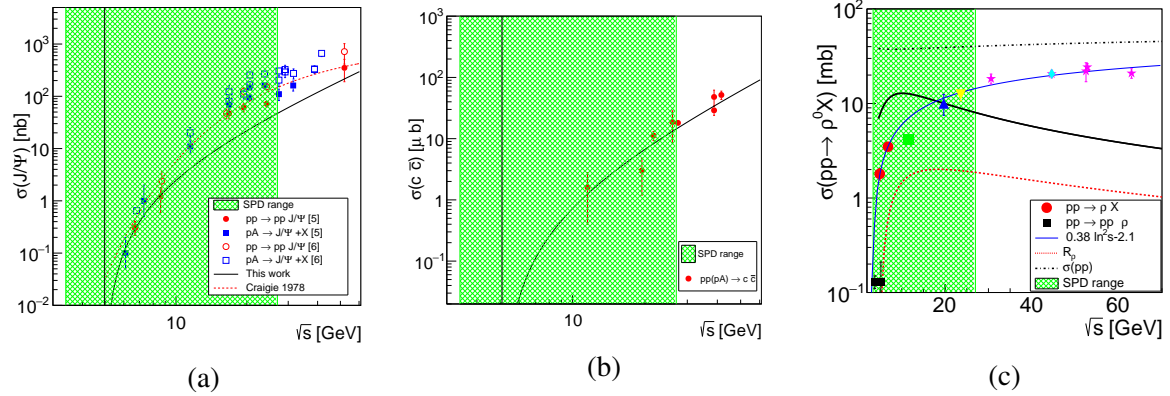
Figure 2.20: (a) Experimental data on J\psi production in p - p (red circles) and p - A (blue squares) reactions, from the recollections in Refs. [277] (filled symbols) and [278] (open symbols). The solid line is the calculation from Ref. [232]. (b) Total charm production in p - p and p - A collisions. The data are from Ref. [282]. The line is a threshold parametrization (see the text). (c) Cross-section for \rho -meson production in p - p collisions: inclusive (different symbols and colors from different experiments) and exclusive data from pp \rightarrow pp\rho (black squares). The present calculation is shown as a black line. The red dashed line is the renormalization factor. The black dash-dotted line is the total pp cross-section. The first red point is the inclusive measurement from Ref. [283]. The blue line is the parametrization from Ref. [284]. The green filled region represents the SPD range.
