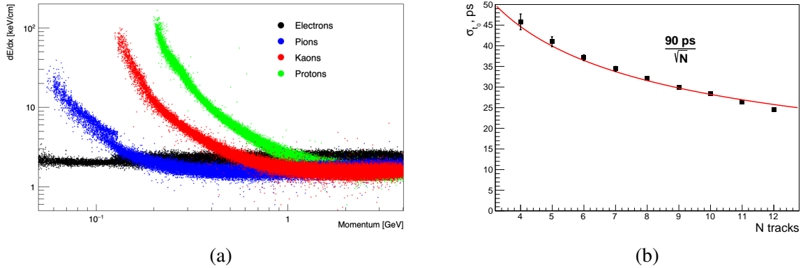
Figure 9.9: (a) Energy deposition dE/dx at the ST for particles emitted at \theta = 90^\circ in respect to the beam axis. (b) Accuracy of the t_0 reconstruction as a function of the number of tracks in the primary vertex.
