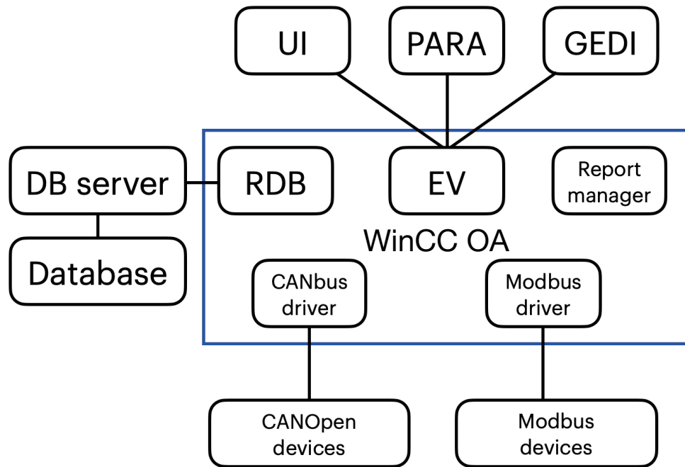
Figure 6.3: SCADA structural scheme of WinCC OA software.
