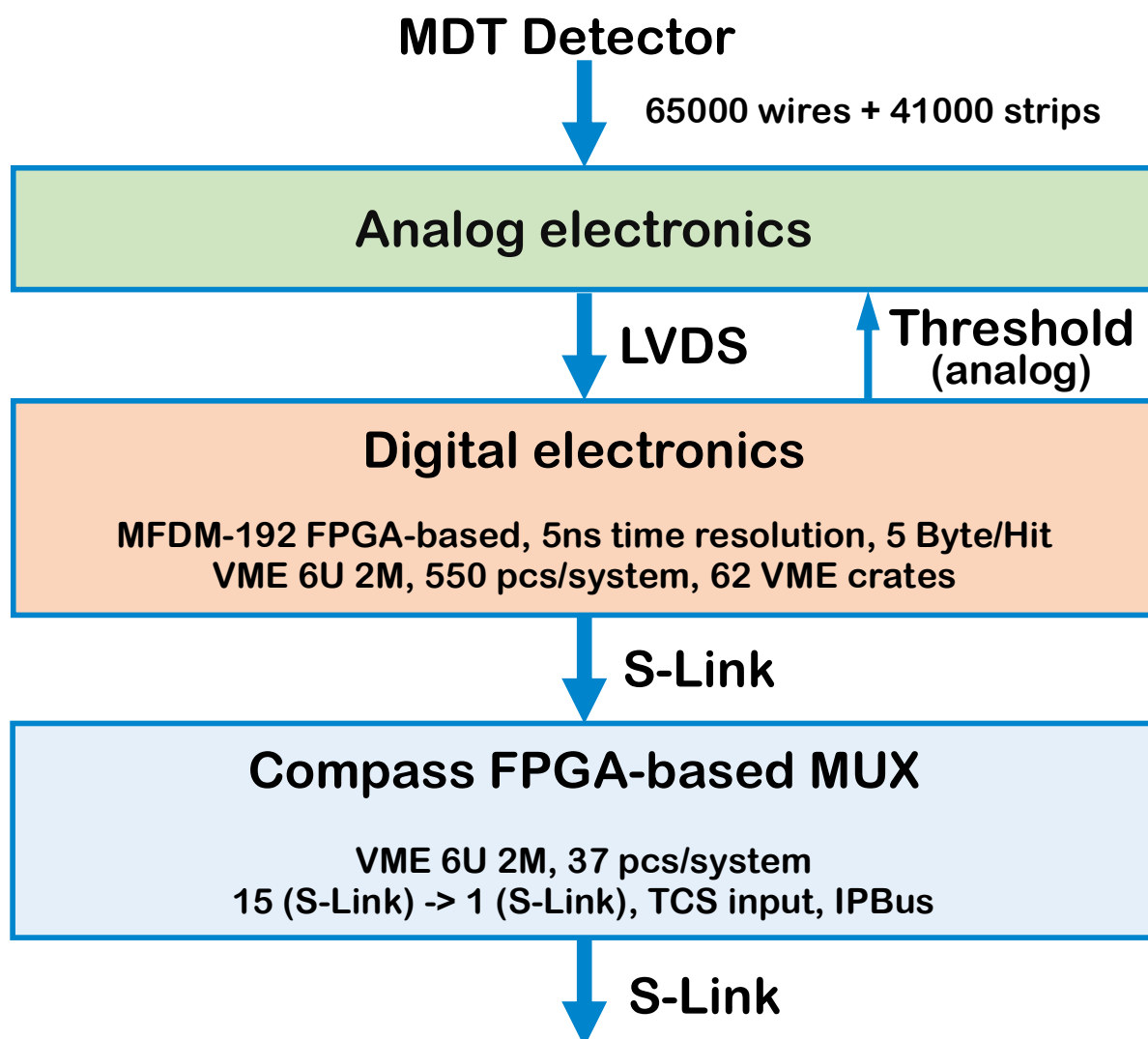
Figure 4.32: Data flow diagram – from detector to DAQ.
