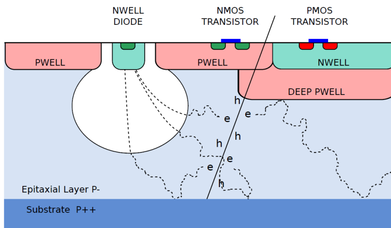
Figure 4.11: Scheme of a MAPS pixel [363].
