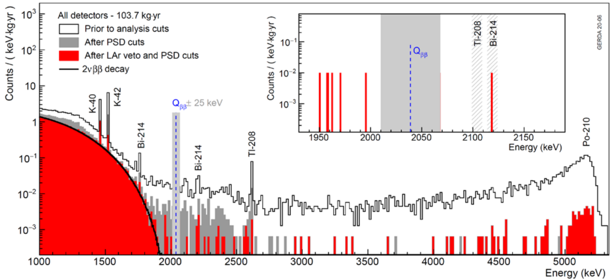
Fig. 3. Final energy PSD spectra of GERDA Phase II. On the inset, the spectrum the spectrum in the ROI is shown. The vertical grey line band shows the blinded region.
