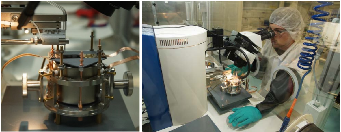
Fig. 7. Left: a detector mount for the GERDA experiment in a protective assembly frame. Right: the wirebond machine used to terminate to the detector for signal and HV.
