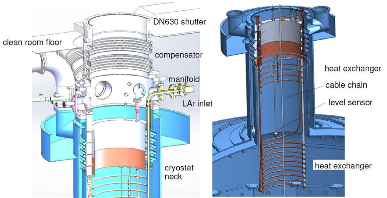
g. 4. Cross section through the cryogenic infrastructure at the cryostat. Left: between the DN630 shutter and the cryostat (compensator and manifold with feedthroughs). Right: inside the cryostat (heat exchanger, fill level measurement).
