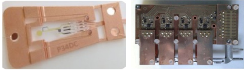
Fig. 10. Photos of Majorana low-mass front-end mounted on an electroformed copper clip (left) and GERDA Phase II charge-sensitive preamplifier (right).
