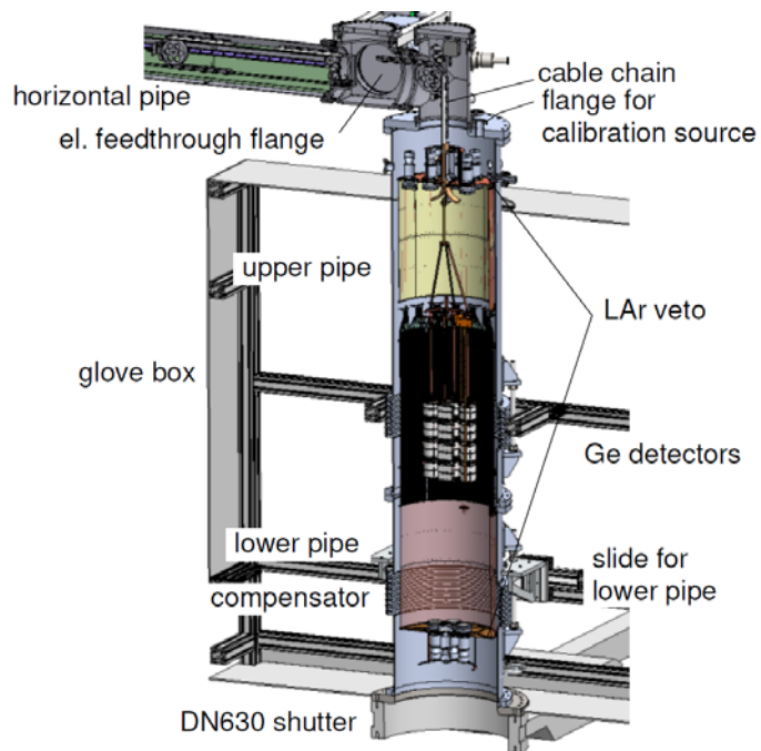
Fig. 5. Schematic cross section of the GERDA lock and glove box. The Ge detector array is in the center surrounded by the LAr veto system. The weight is supported by the cable chain. The vertical lock is separated into an upper and a lower pipe. Both can be compressed due to compensators and the lower one then slides to the side inside the glove box to open the lock.
