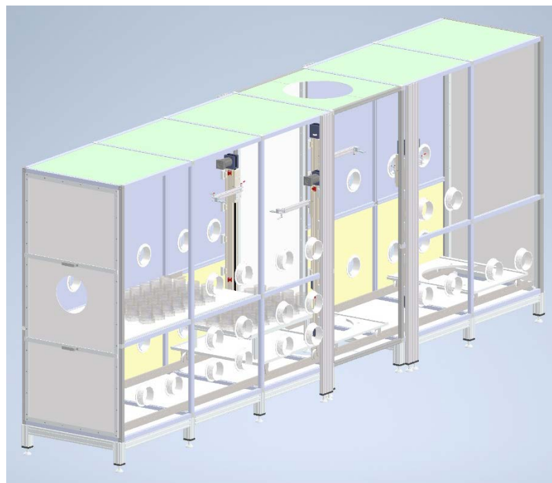
Fig. 9. Design of the glove box for LEGEND-200.
