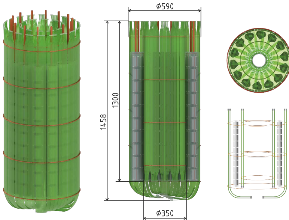
Fig. 12. Latest design of LEGEND-200 LAr veto system, developed by JINR and TUM specialists.
