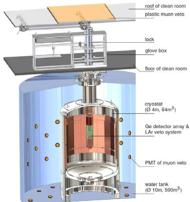
Fig. 1. Schematic cross section of the GERDA experiment. The main components are labelled.
