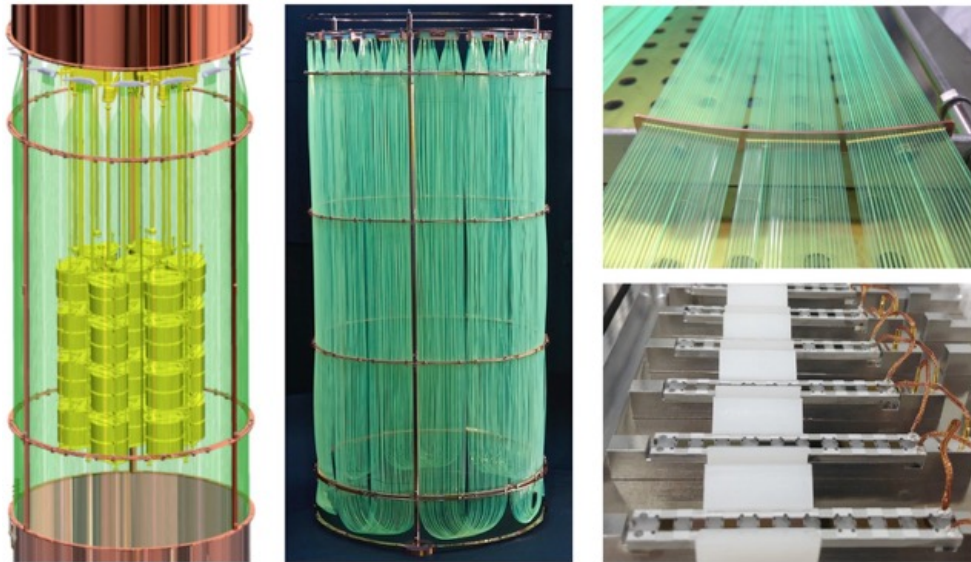
Fig. 11. Wavelength shifting (WLS) fiber shroud with SiPM readout of GERDA. Left: artist's view with germanium detector array; middle/right top: photo of WLS shroud during production; right bottom: SiPMs in die mounted on micro-machined fused quartz substrates. All materials are selected and screened for their intrinsic radio purity.
