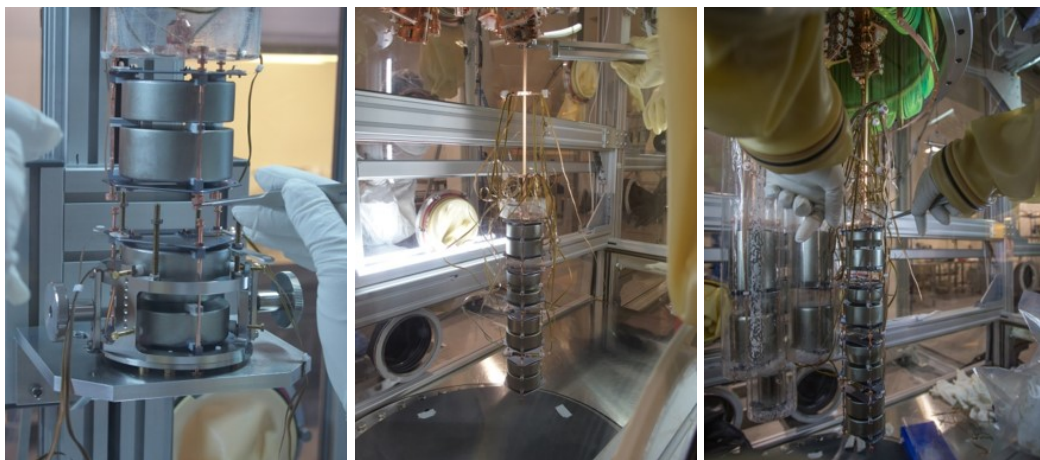
Fig. 8. The GERDA string building process.
