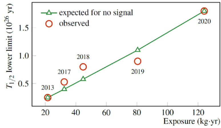
Fig. 14. Increase of sensitivity with exposure measured in the GERDA experiment.
