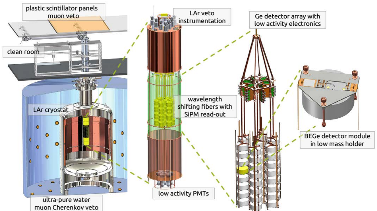
Fig. 6. Detector mounts, strings and LAr veto for the GERDA experiment.
