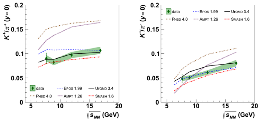
Fig.1. Comparison of the energy dependence of K^+/\pi^+ (left) and K/\pi^- (right) yields ratio at mid-rapidity for the 20% most central Be+Be collisions with models: EPOS 1.99 (blue dashed line), UrQMD 3.4 (black solid line), AMPT 1.26 (violet dotted line), PHSD (brown dashed-dotted line) and SMASH 1.6 (red dashed-double dotted line).
