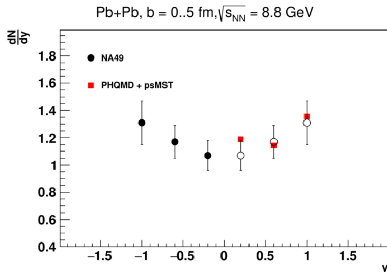
Fig.2. Rapidity spectra of deuterons measured in central Pb+Pb interactions at 40 GeV/c. Experimental data are shown with black circles, PHQMD + psMST predictions with red squares.
