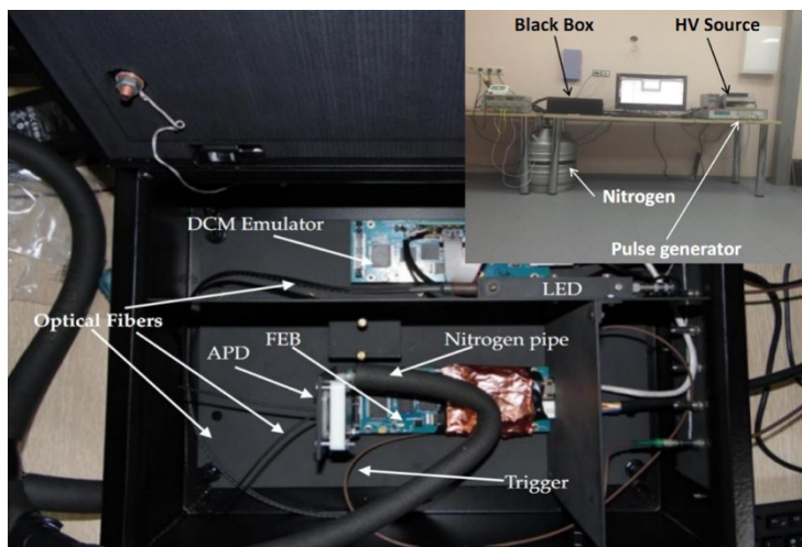
Figure 35. NOvA test bench.
