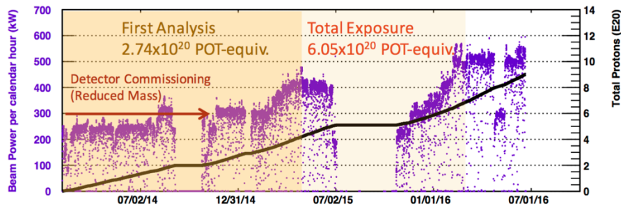
Figure 4. Integrated POT flux and NuMI beam power.
