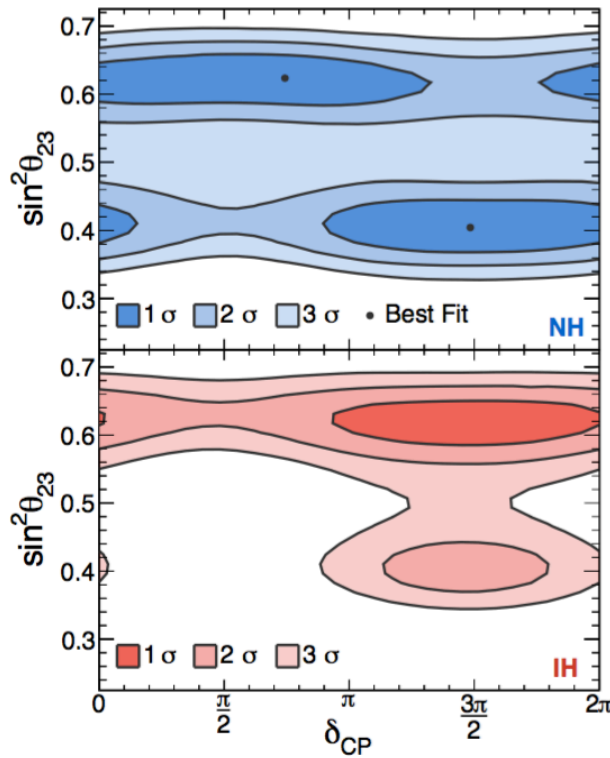
Figure 25. 1, 2 and 3 \sigma allowed regions using \nu_{\mu e} constraint in \sin^2\theta_{23} vs \delta_{CP} for normal (top) and inverted (bottom) hierarchy. No Feldman-Cousins corrections are applied.
