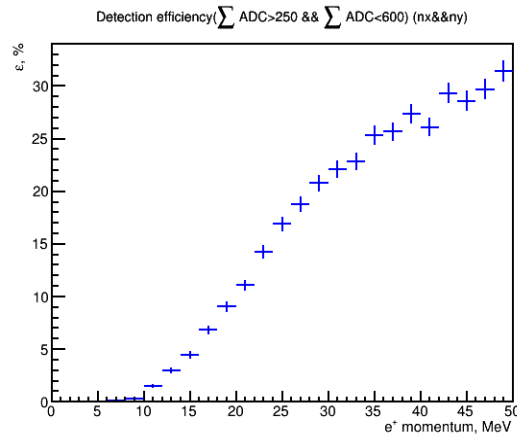
Figure 48. Efficiency of positron detection depending on positron momentum (right).
