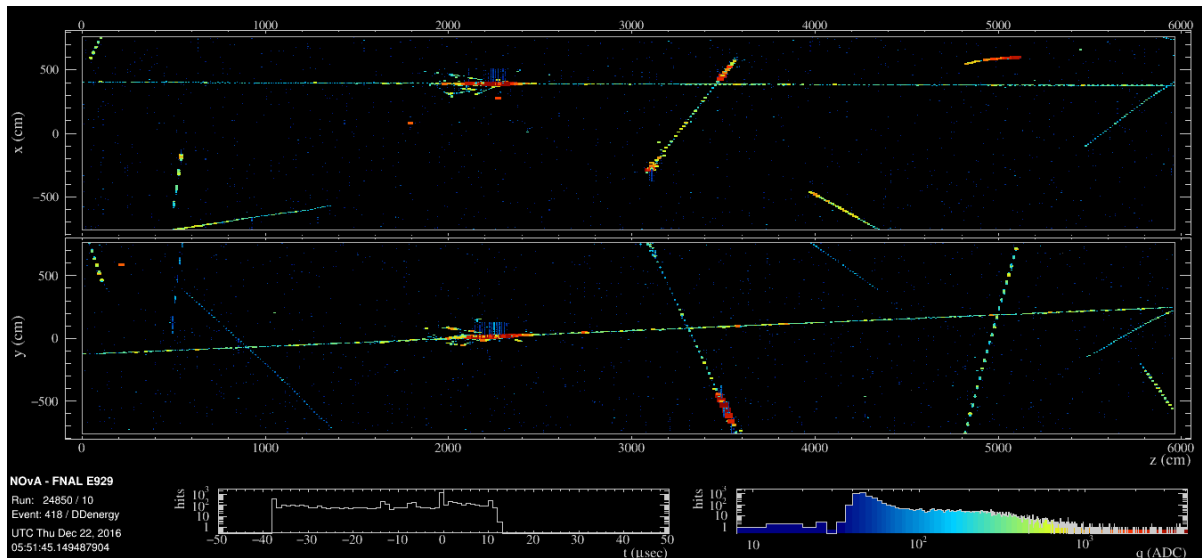
Figure 58. High-energy muon in real data of the Far Detector of NOvA.
