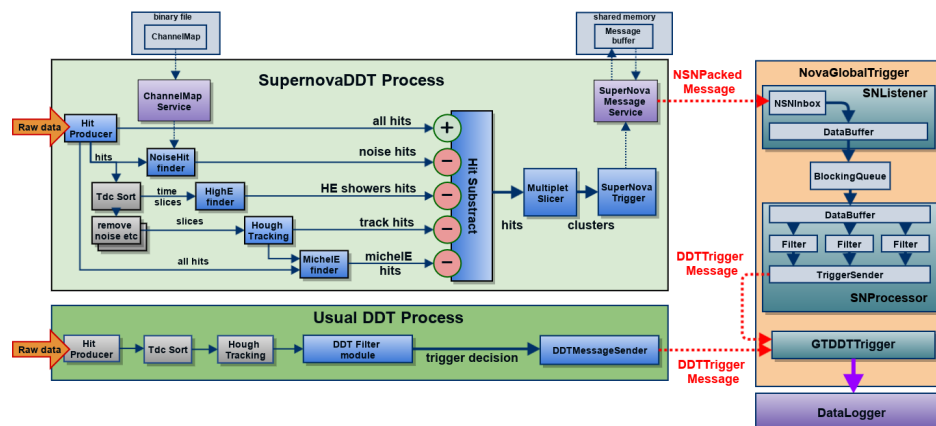
Figure 49. Scheme of Supernova DDT process in comparison with usual DDT trigger.
