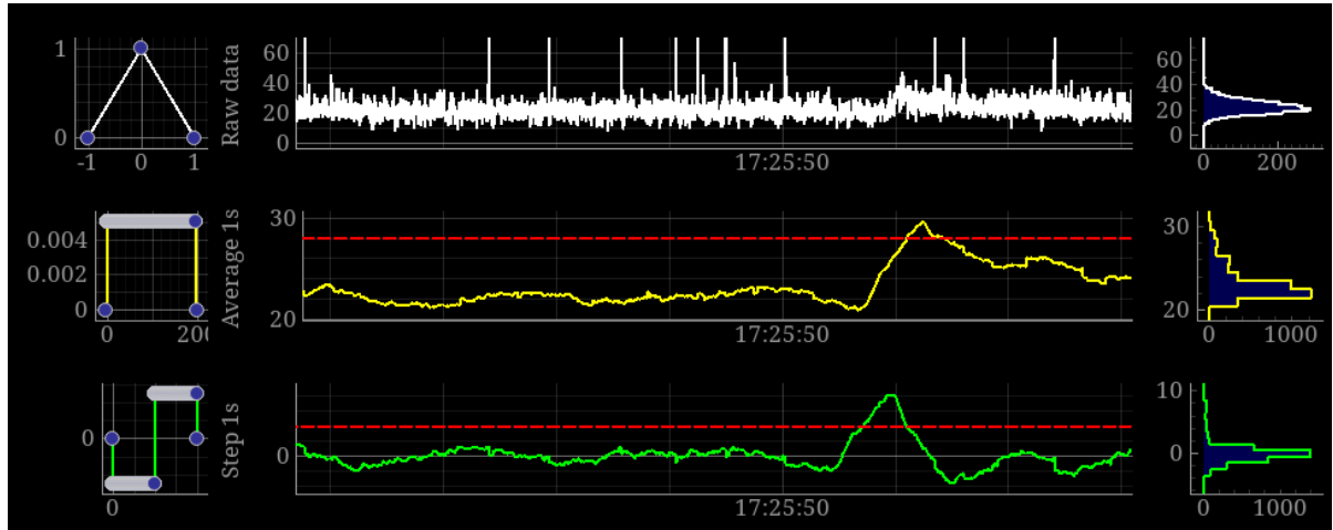
Figure 50. Example of supernova signal detection using filters to enhance the signal.
