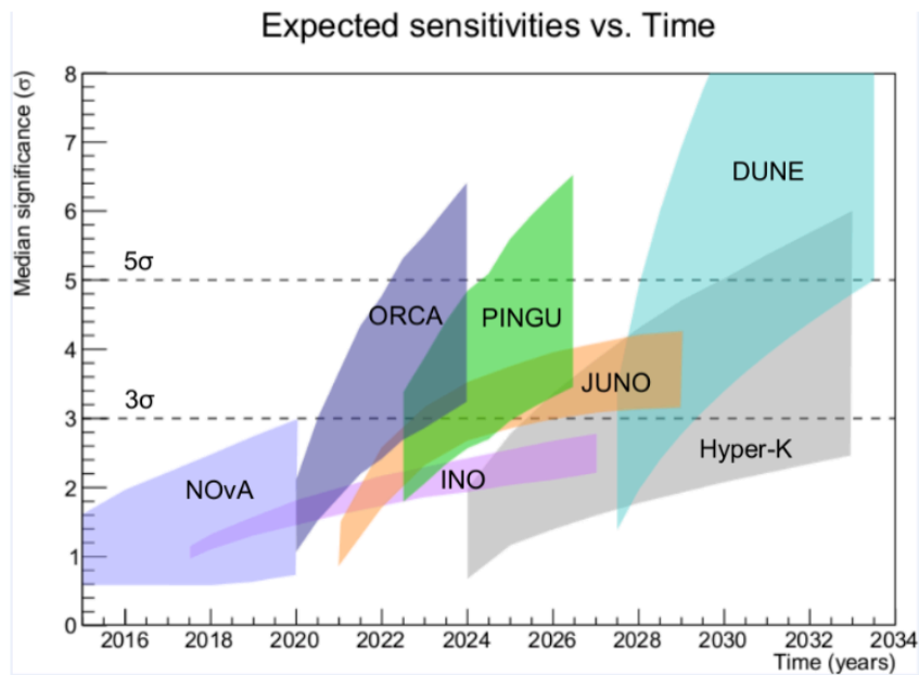
Figure 29. Expected time scale sensitivities for going and future neutrino experiments.
