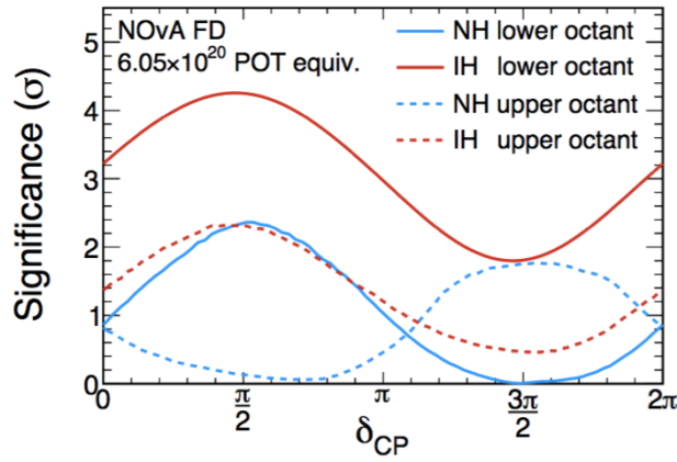
Figure 26. Significance as a function of \delta_{CP} for NH (blue) and IH (red), with fixed \sin 2\theta_{23}=0.4 (solid) and \sin 2\theta_{23}=0.6 (dotted). Feldman-Cousins corrections are applied. Signal and background systematics are taken into account. \Delta m_{21}^2 and \sin 2\theta_{13} are held within global uncertainties.
