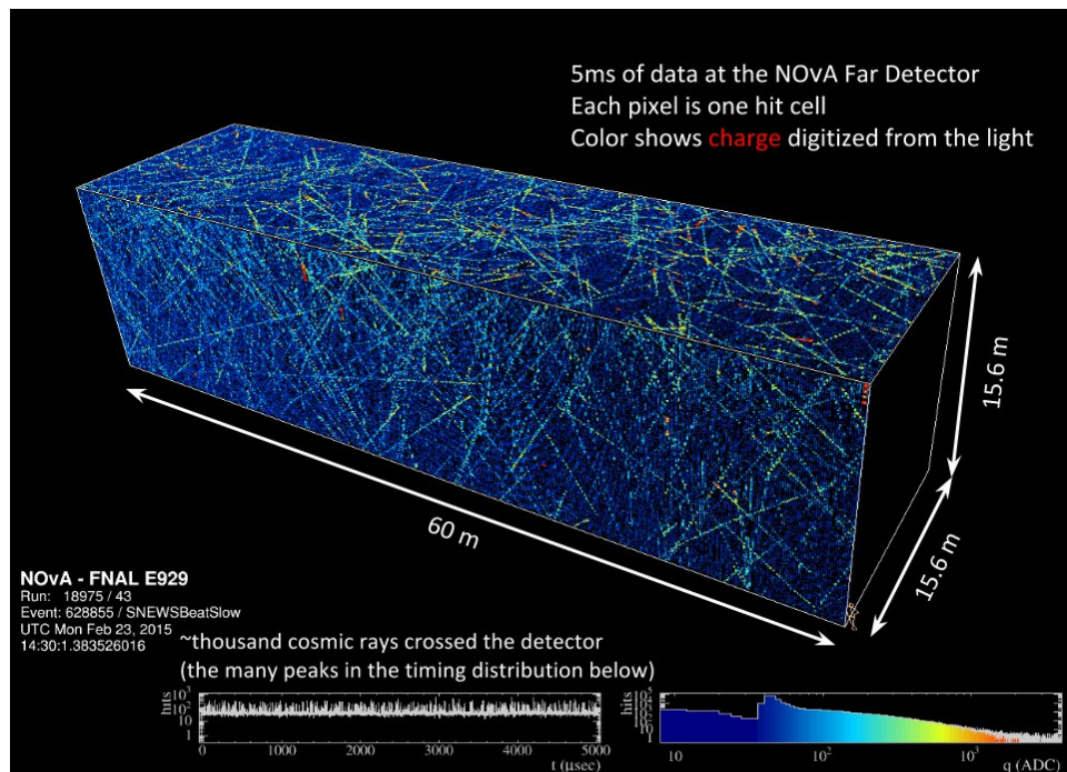
Figure 53. Event display of NOvA Far Detector with many cosmic ray tracks.
