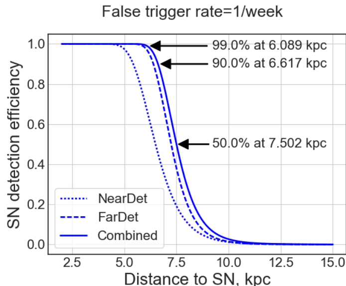
Figure 51. Supernova detection efficiency on a distance from supernova explosion.
