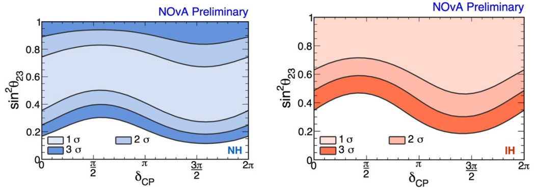
Figure 24.1, 2 and 3 \sigma allowed regions in \sin^2\theta_{23} space for normal (left) and inverted (right) hierarchy, as a function of \delta_{CP} . No Feldman-Cousins corrections are applied. Signal and background systematics are taken into account.
