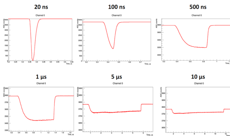
Figure 38. PMT signals on stand-alone ADC.
