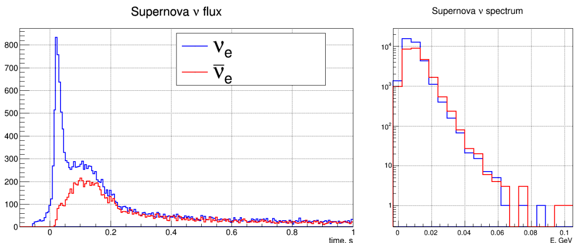
Figure 46. Neutrino composition and spectra from supernova explosion.
