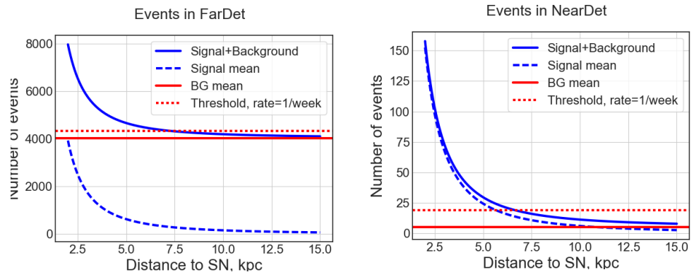
Figure 52. Event rates for signal and background.
