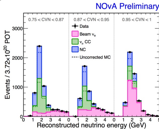
Figure 19. Reconstructed neutrino energy spectra of ND events for different PID bins after tuning.
