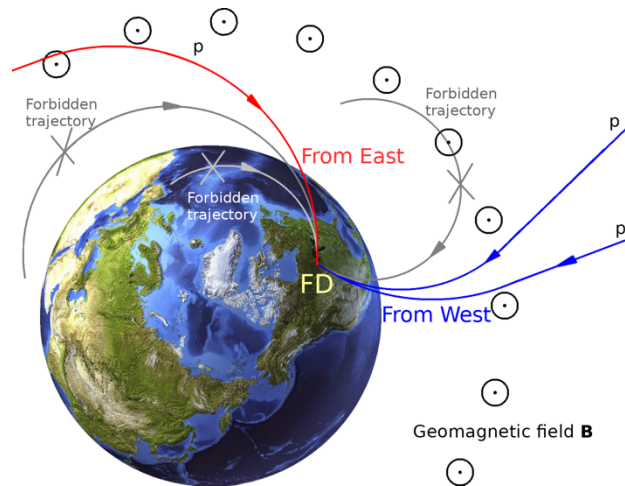
Figure 54. East-west asymmetry of cosmic rays for NOvA FD.
