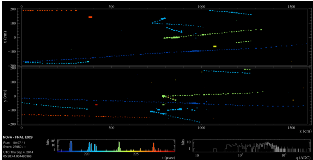
Figure 62. A NOvA Near Detector event with three muon tracks from the rocks and two neutrino interactions, this shows the capabilities of the NOvA Near Detector.
