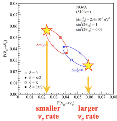
Figure 22. Oscillation probabilities in NOvA case. The blue curves are for the normal hierarchy and the red curves are for the inverted hierarchy. On each ellipse, the choice of the CP phase delta varies as one moves around the ellipse as indicated by the symbols. This assumes maximal maxing in the theta_23 octant. Stars are corresponded to smaller/larger nue rates (and opposite in antimue case).
