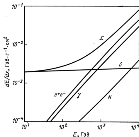
Figure 57. Energy loss components of muon (in iron). This picture is borrowed from [16].
