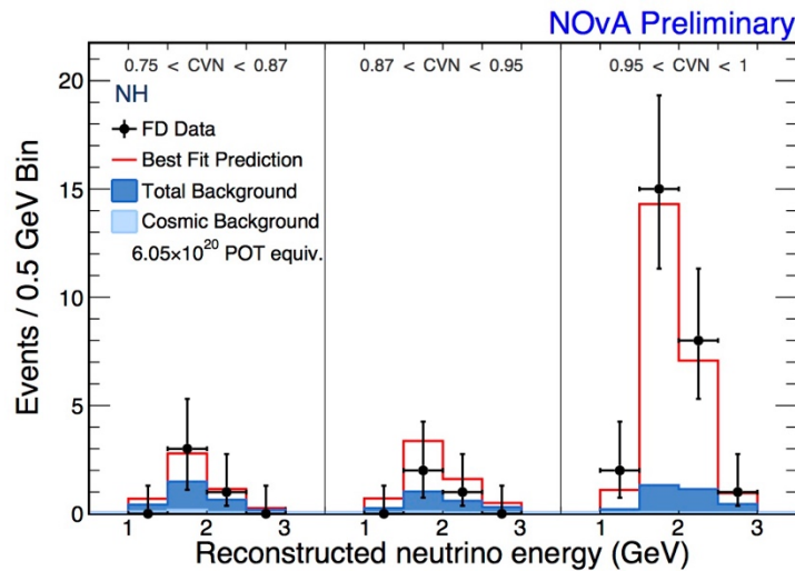
Figure 23. Nue SA Energy vs PID distribution of FD selected events in data and MC prediction. This MC prediction uses the best fit parameters for Normal Hierarchy.
