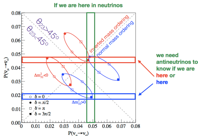
Figure 27. NOvA \nu_{\mu e} Bi-probabilities splited by \theta_{23} octant non-maximal values.
