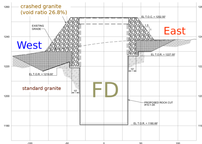
Figure 55. Asymmetry of the hill around Far Detector.
