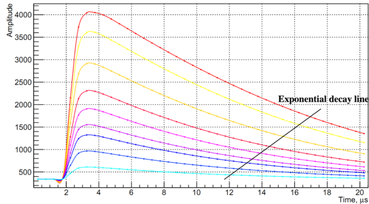
Figure 40. APD signals with different amplitudes.
