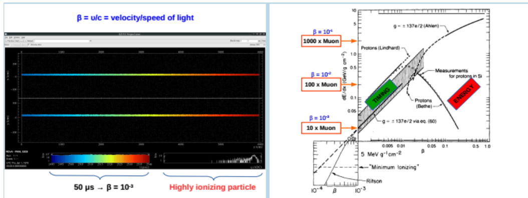
Figure 59. Simulated monopole in Far Detector (left) and monopole energy loss depending on its beta (right).
