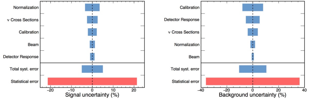
Figure 20. Signal (left) and background (right) uncertainties.
