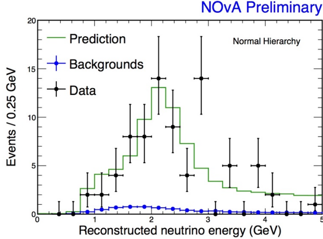
Figure 10. SA numu final spectrum showing data and best fit prediction.
