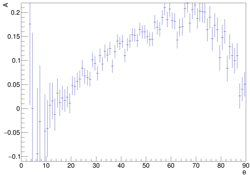
Figure 56. East-west asymmetry of cosmic-ray muons, stopped in the Far Detector of NOvA, without hill asymmetry correction. Asymmetry is defined as A=(W-E)/(W+E) , where W is cosmic muon flux coming from west, E is one from east.
