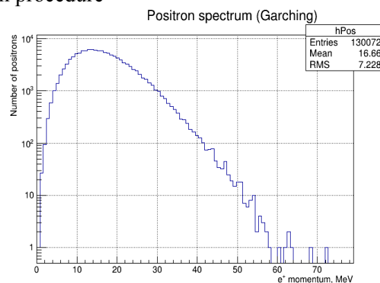
Figure 47. Positron spectrum from supernova IBD interactions
