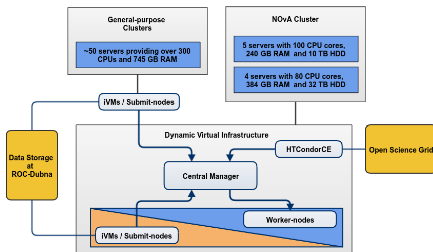
Figure 44. The scheme of the cloud infrastructure.
