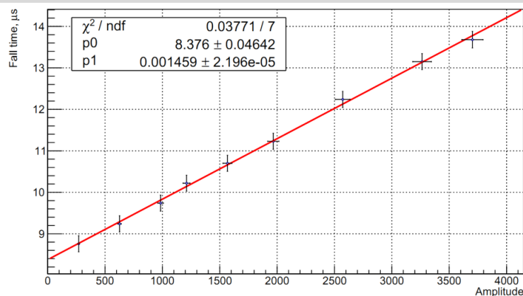
Figure 41. Fall time dependence on the amplitude of the signal.
