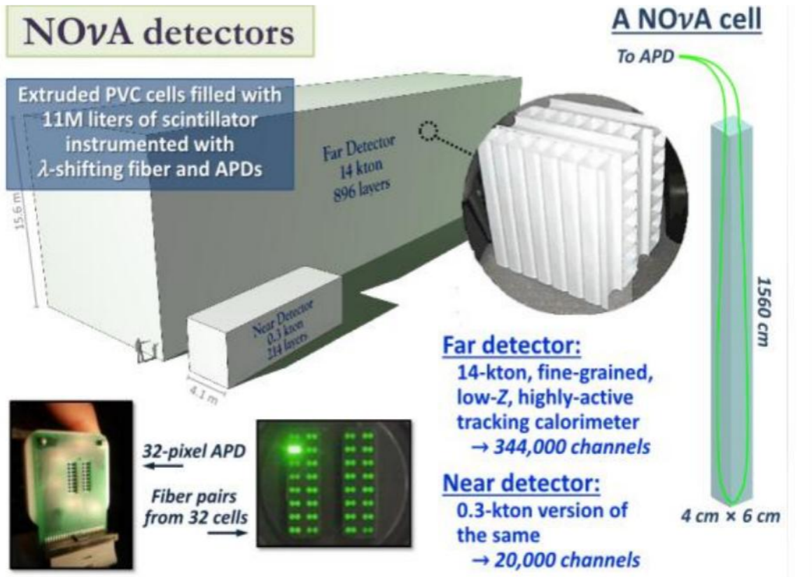
Figure.2. General concept of the NOvA detectors design
