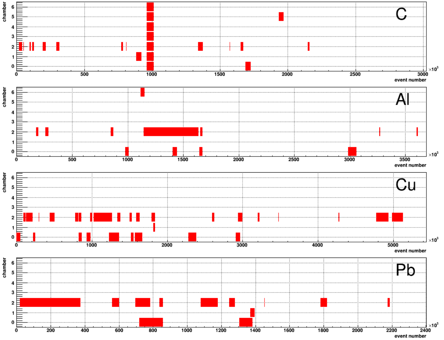
Рис. 2: T=4.5 GeV
