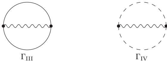
Figure: Two-loop Feynman supergraphs with hypermultiplet and ghosts vertices.
