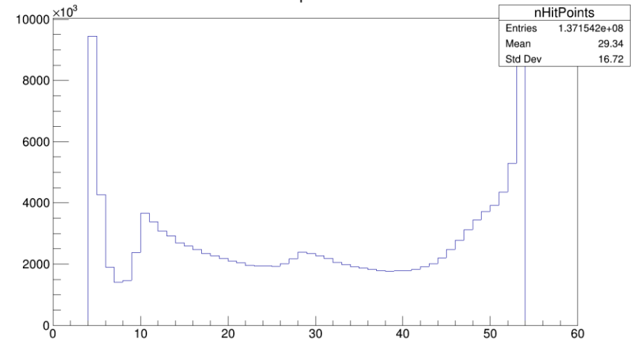
Number of hit points distribution
