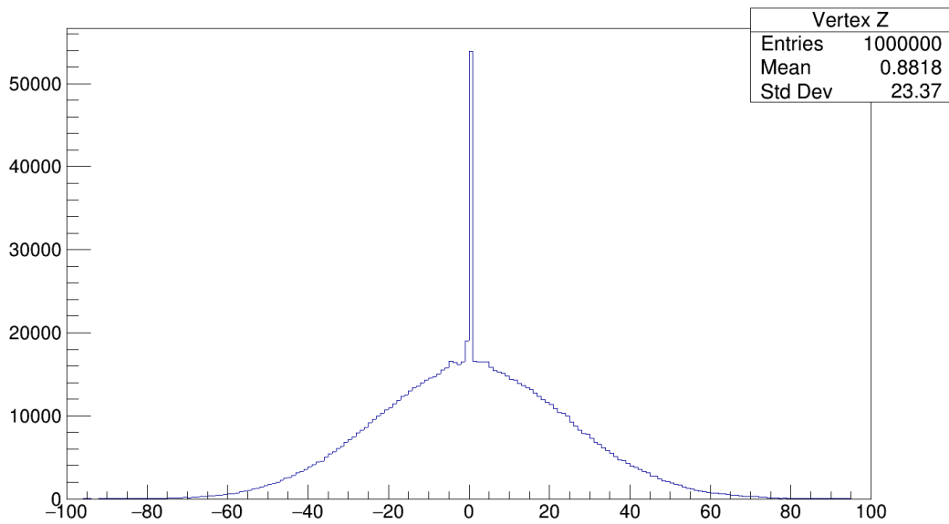
Vertex Z distribution
