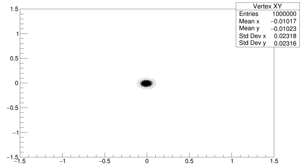
Vertex XY distribution
