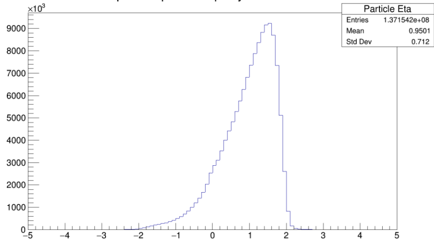
particle pseudorapidity distribution
