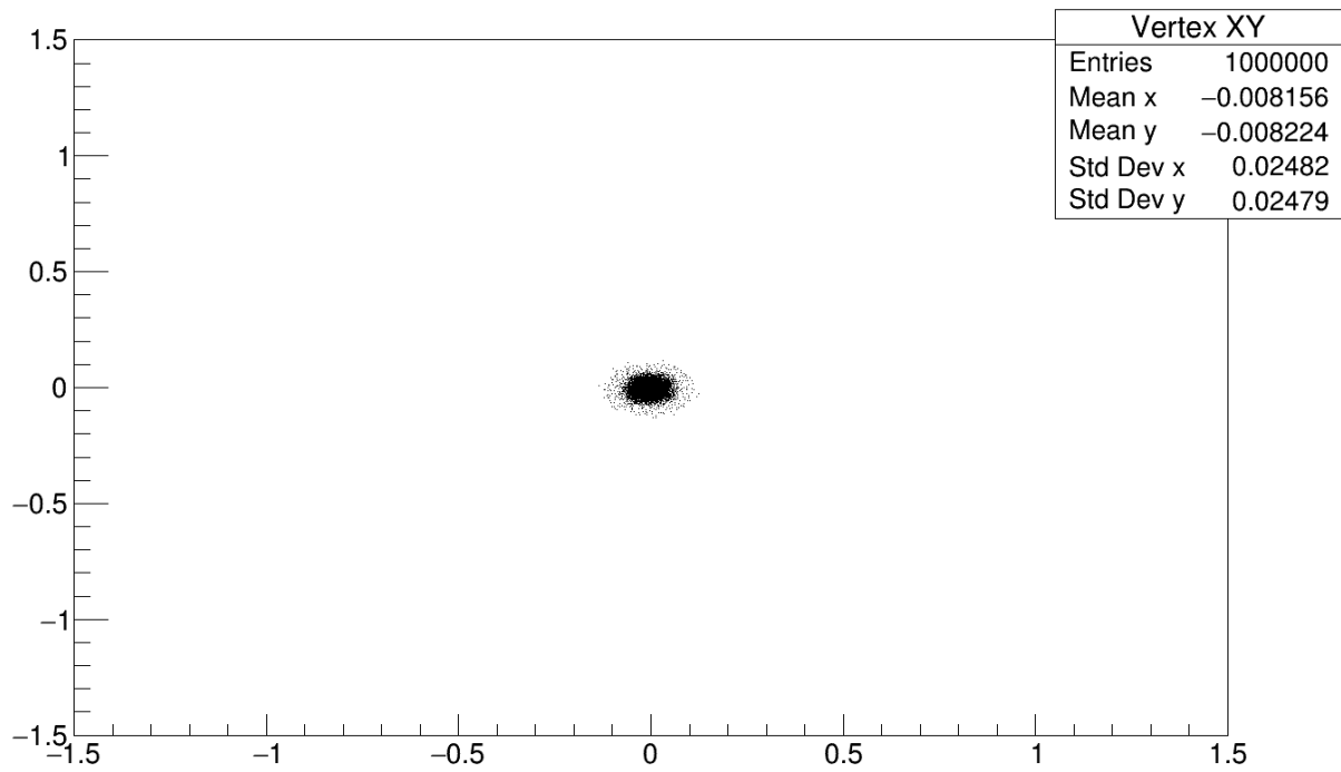
Vertex XY distribution
