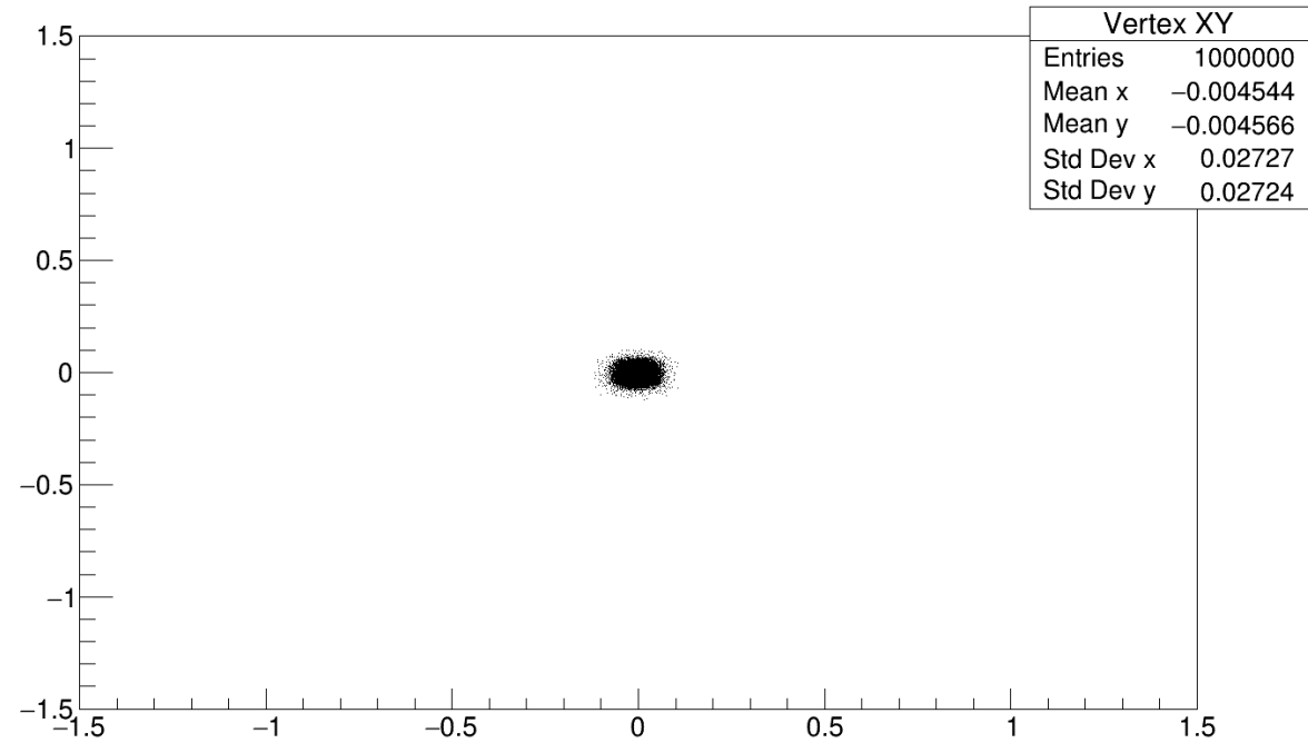
Vertex XY distribution
