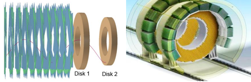
Fig. 3.5.1: a) 3D view of the Mu2e detector showing the straw tracker and the electromagnetic calorimeter, along with the track of a conversion electron. b) CAD drawings of the calorimeter disks. Calorimeter innermost (outermost) radius is of 351 mm (670 mm) with a crystal length of 200 mm. Layout of the FEE and digitization crates is also shown.
