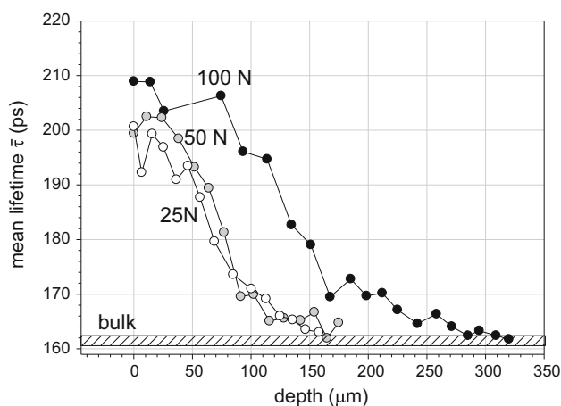
Fig. 3 Values of the mean positron lifetime as a function of depth from the worn surface of pure Zr sample. The sample was exposed to sliding against the rotating martensitic steel disc with different loads of 25, 50 and 100 N during the time of 1 min
