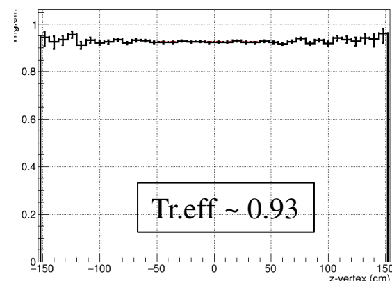
FFD||FHCAL trigger efficiency vs. z-vertex
