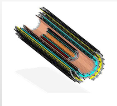
MPD ITS based on ALICE type staves
