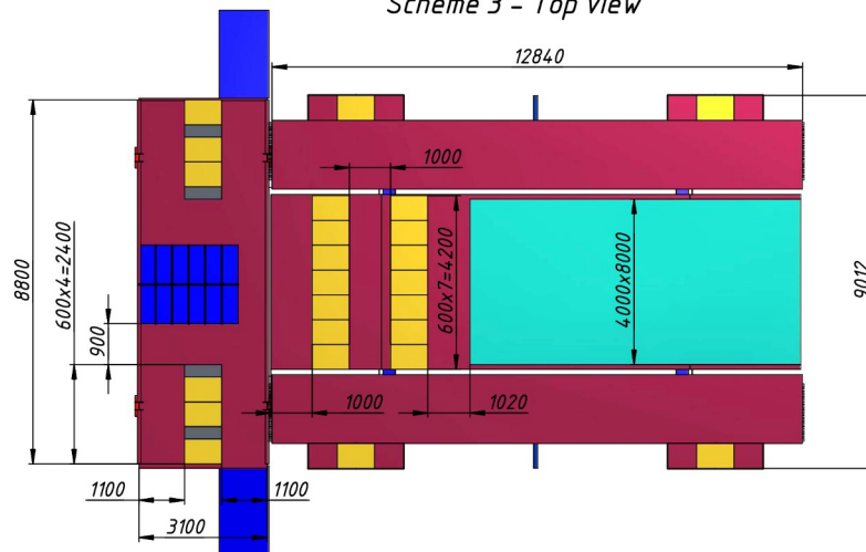
Scheme 3 - Top view
