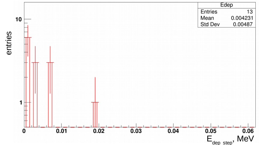
total deposited energy (MeV)
