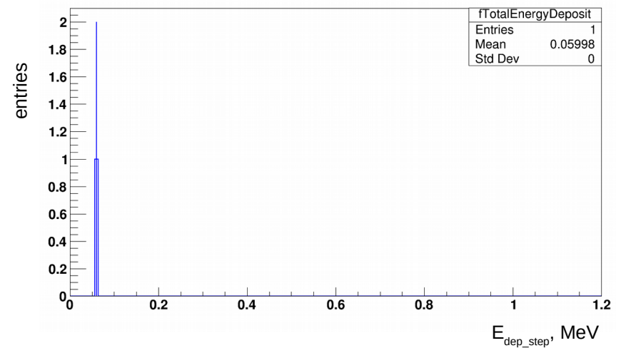
total deposited energy (MeV)
