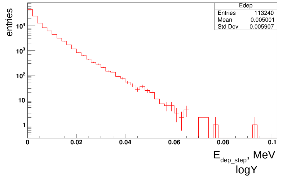
hit deposited energy (MeV)
