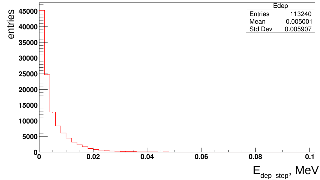
hit deposited energy (MeV)
