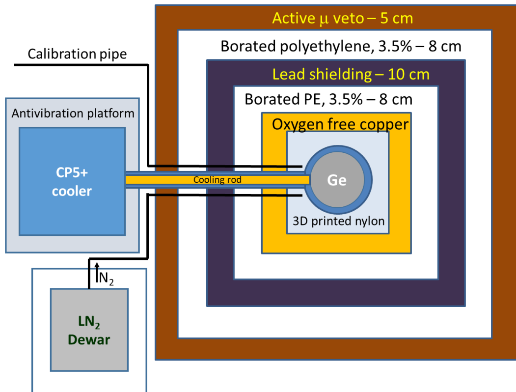
Pic.1. Scheme of the vGeN shielding. Top view [1].
