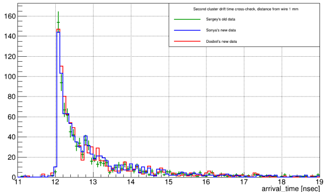
Second cluster drift time compare, distance from wire 1 mm
