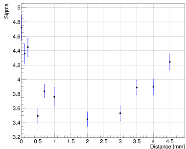
New Sigma from distance to wire
