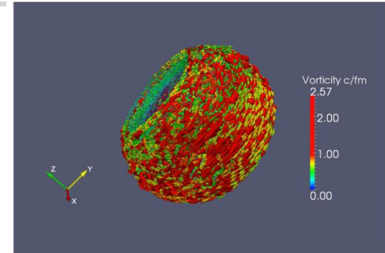
FIG. 3. The vortex sheet.
