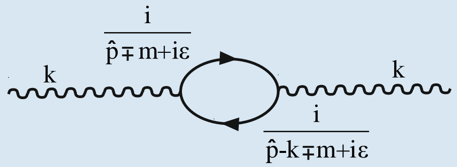
Fig. 4. Feynman diagrams in the second order of perturbation theory
