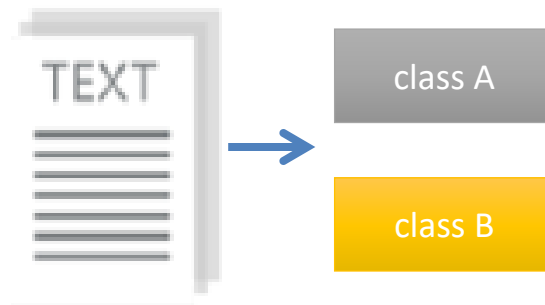
Classification
