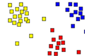
Clustering
