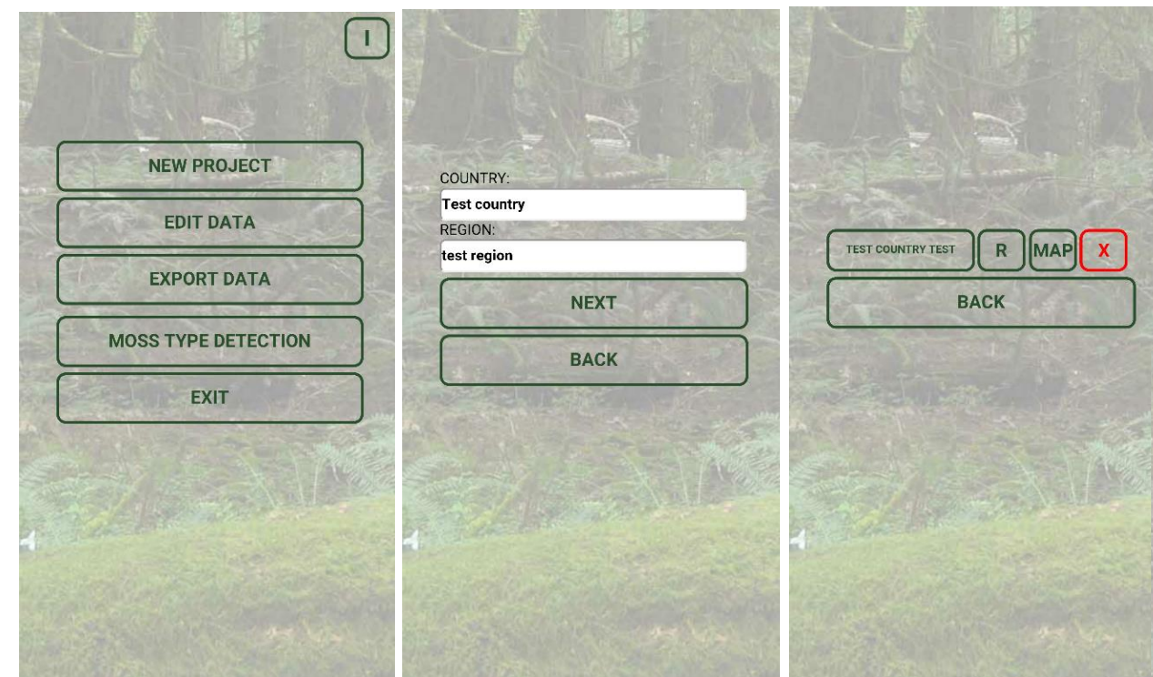
Create/edit project
