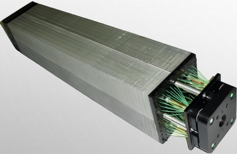
Fig. 11. ECal module photo without light shielding cover
