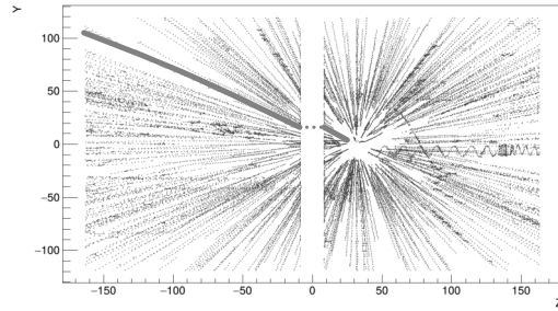
Fig. 5: Explanation of the algorithm of trigger latency calculation based on linking of tracks crossing HV electrode
