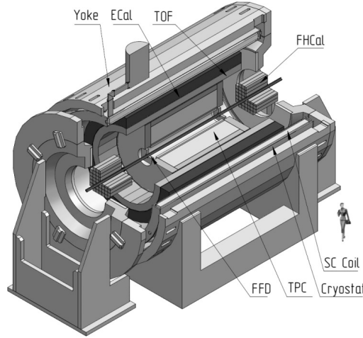
Fig. 1: NICA MPD 1-st stage setup
