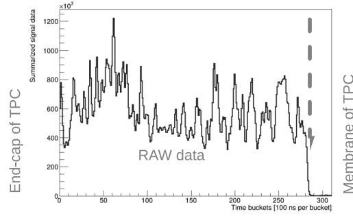
Fig. 4: Position of HV electrode on summarized raw data signal
