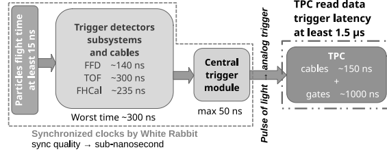
Fig. 2: MPD trigger flow diagram
