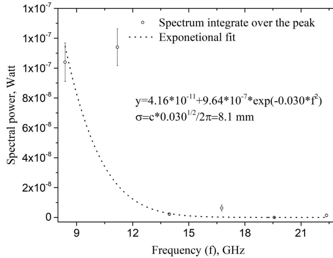
Fig. 3. — Determination of the length of the electron bunch: points are the frequency spectrum for 3 rd to 8 th harmonics; the dashed curve is an exponential fit function.
