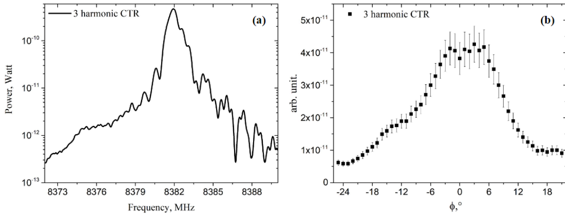
Fig. 2. — a) The spectrum of the 3 rd harmonic CTR; b) The orientation dependence of the 3 rd harmonic CTR.
