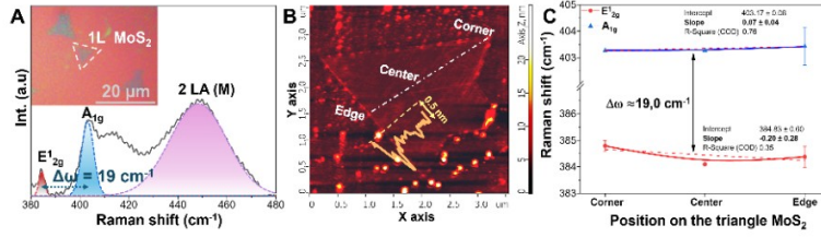
Figure 1. (a) Raman spectra of monolayer MoS 2 under 633 nm laser excitation, inset of the brightfield optical micrograph on MoS 2 deposited on silicon surface, (b) AFM image of a monolayer MoS 2 . Inset: the height profile along the dashed line and the dash-dot line to denote the measured Raman positions, (c) the vibrational modes A 1g , E 12g 1 , shifts in dependence of the position from corner to edge of the triangle MoS 2 .
