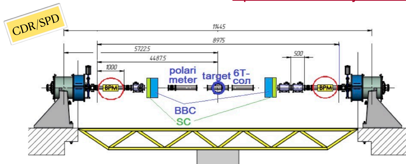
Figure 11.2: The SPD straight section equipped with the diagnostic and control units. All dimensions are in millimeters.
