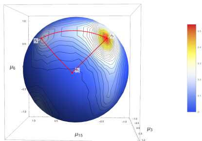
Figure 5: The probability distribution of 2-qubit SW kernels over the moduli space of qutrit.
