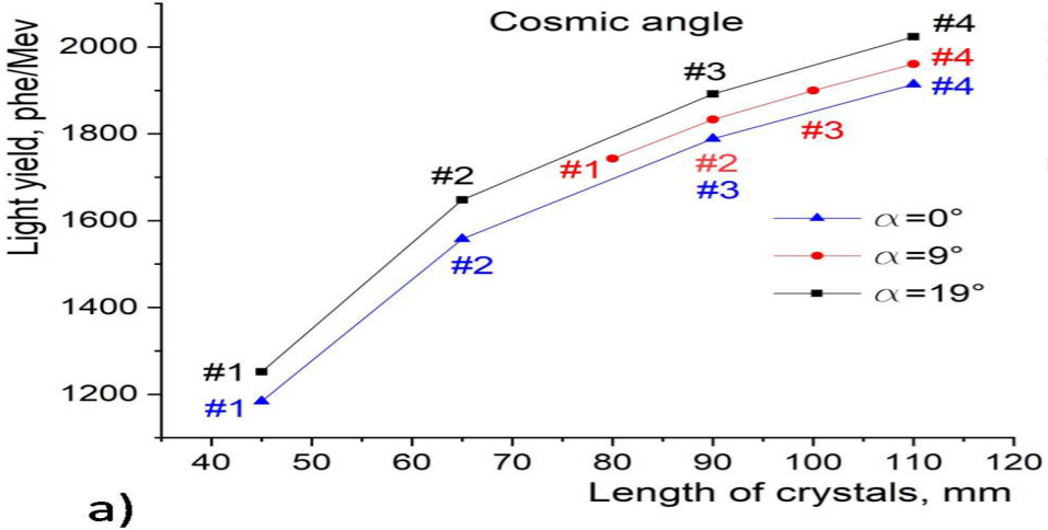
a) Scintillator responses of the calorimeter prototype for angles of 0, 9 and 19 degrees ; b) Detector response non-uniformity for angles 0, 9 and 19 degree
