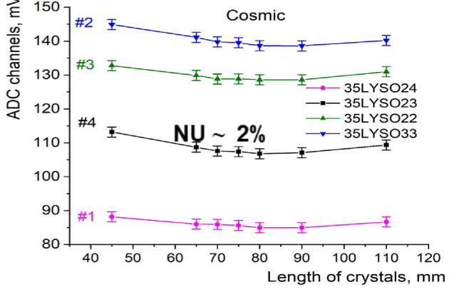
Non-uniformity of the prototype response along the crystals measured using cosmic muons
