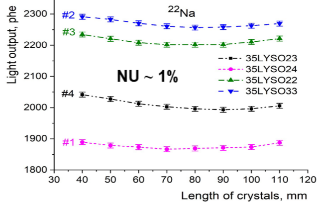
Non-uniformity of the LY along the crystals length, measured at an energy of 511 keV
