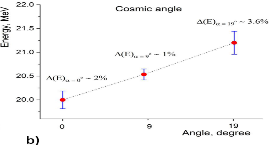
a) Scintillator responses of the calorimeter prototype for angles of 0, 9 and 19 degrees ; b) Detector response non-uniformity for angles 0, 9 and 19 degree
