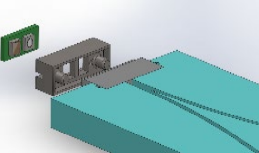
Sketch of the strip with SiPM board and housing. The real look of the SiPM PCB inserted to the housing
