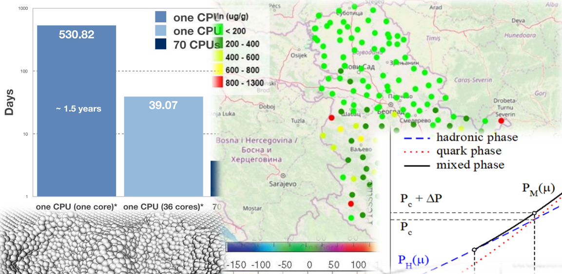
Govorun Supercomputer
