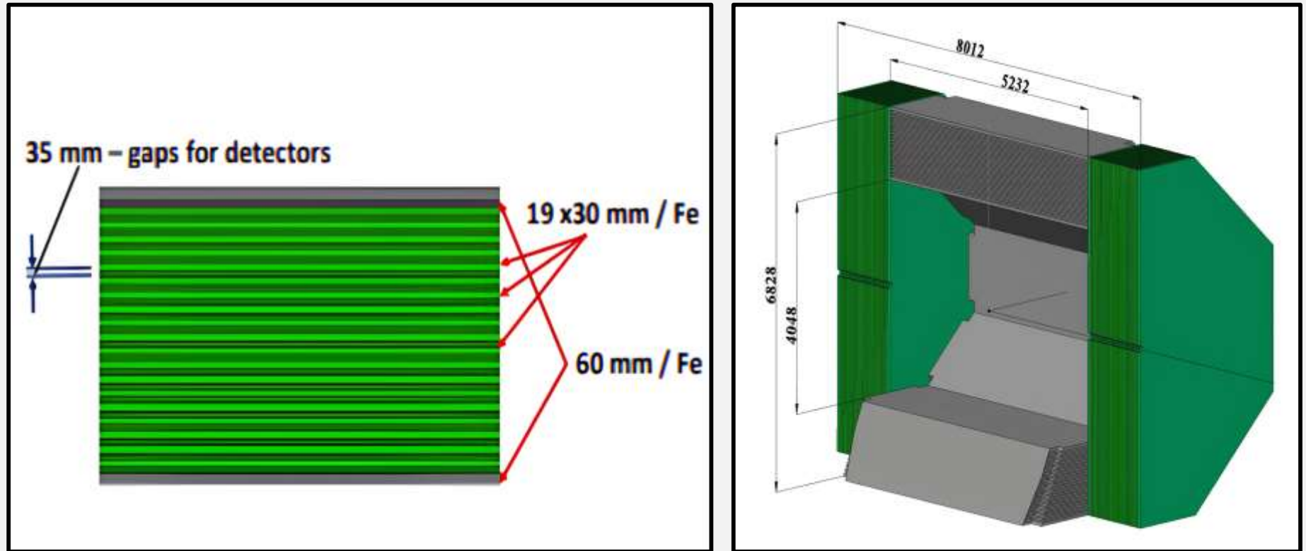
Fig. 2 Left - cross section of the detecting parts of the range system, right - schematic view of the system
