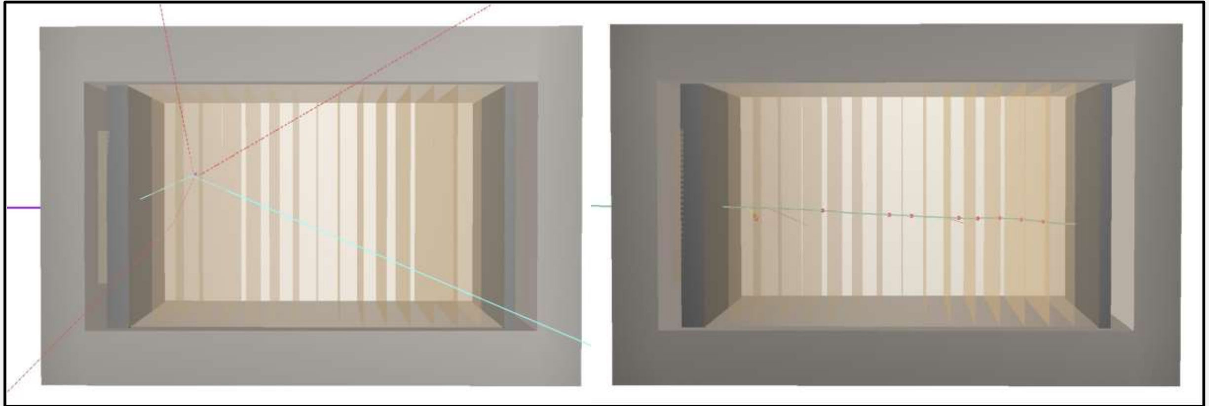
Fig. 5 Passage of a proton and a muon with an energy of 1 GeV through the prototype Left – proton, right – muon
