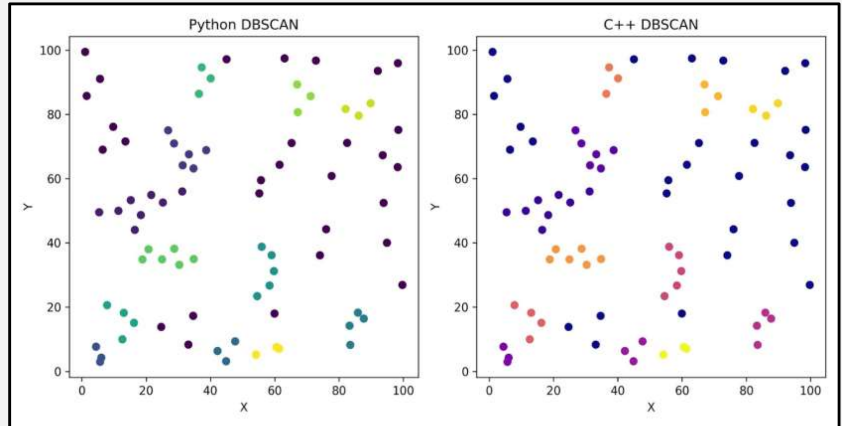
Fig. 8 Results of the DBSCAN algorithm in python and C++ implementations compared
