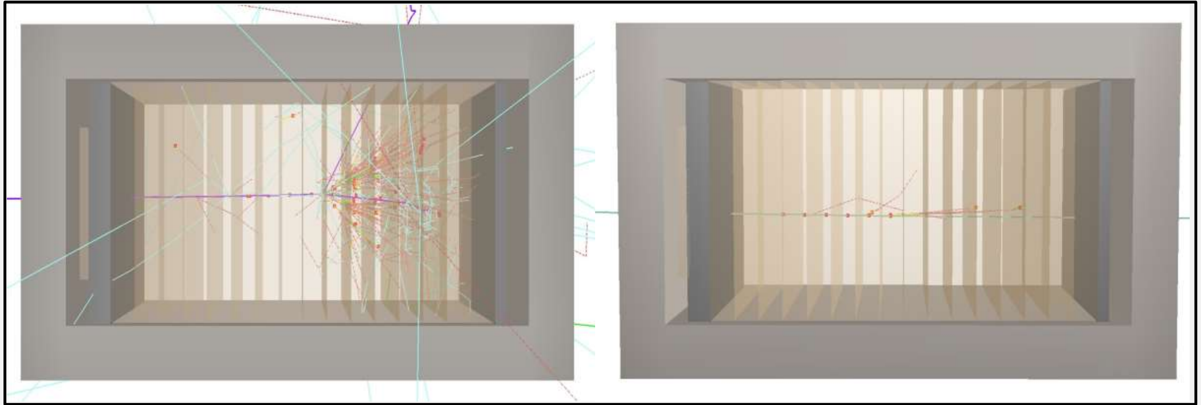
Fig. 6 Passage of a proton and a muon with an energy of 10 GeV through the prototype Left – proton, right – muon
