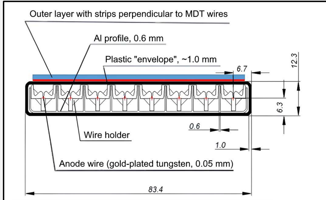
Fig. 3 Left - cross section of the MDT detector, right – the real prototype
