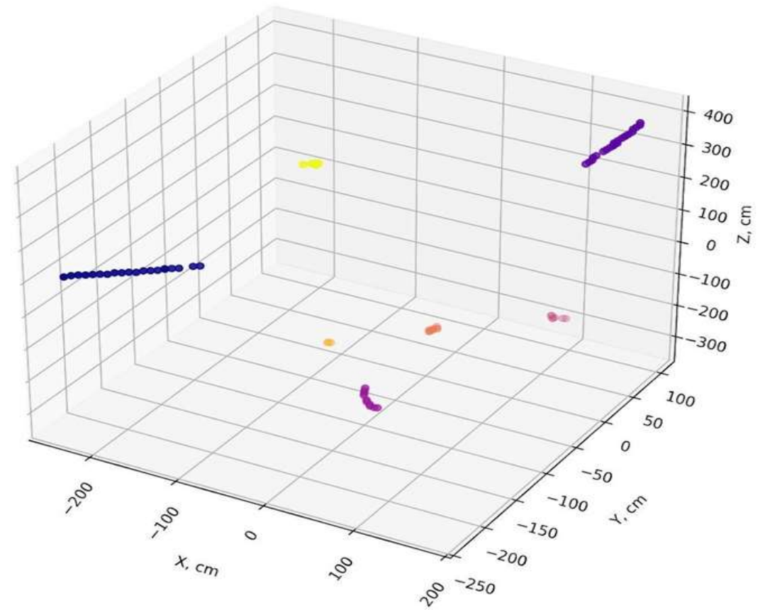
Fig. 9 Visualization of point clustering in one of the events for J/\psi
