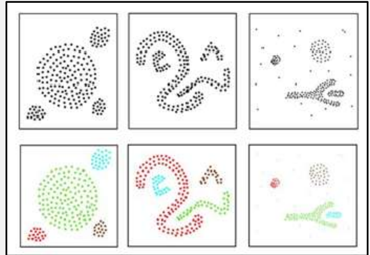
Fig. 7 Illustration of how DBSCAN works
