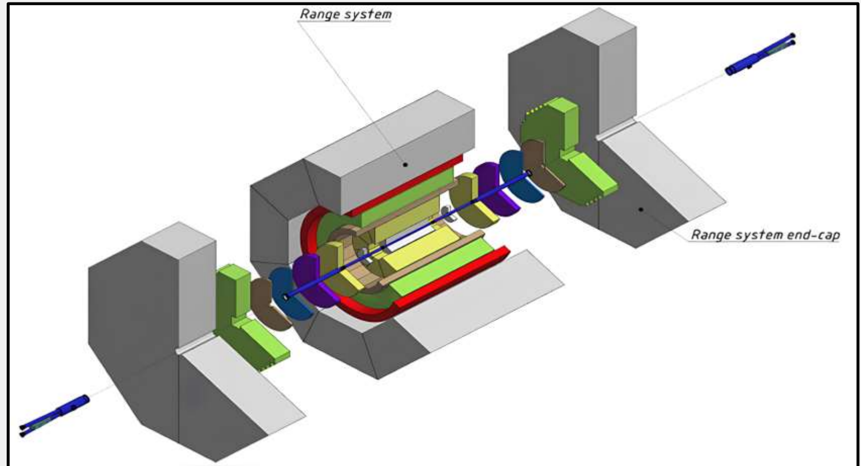
Fig. 1 The range system in the SPD setup
