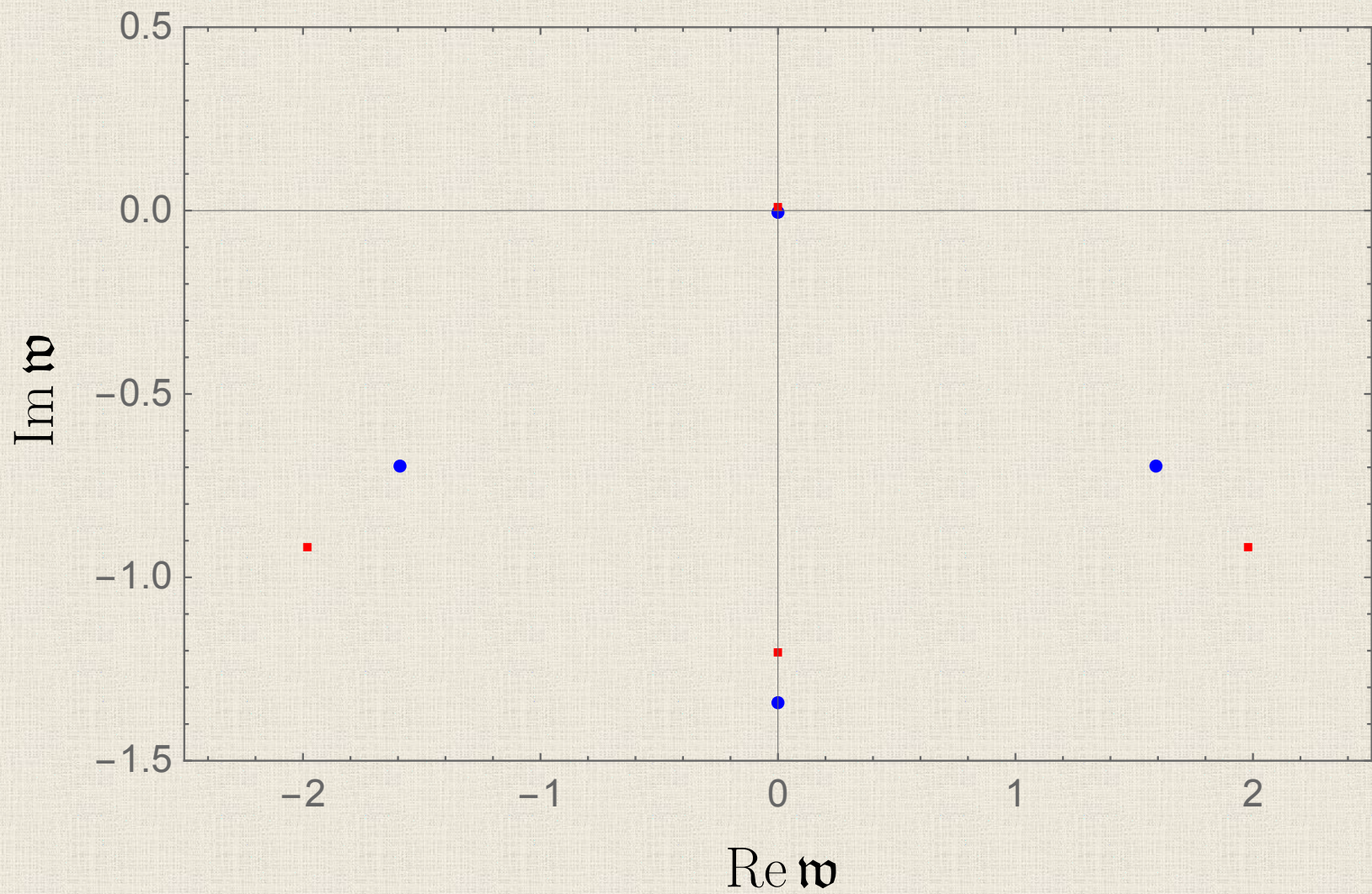
The spectrum of linear fluctuations in the complex frequency plane for k < 1 (blue) and k > 1 (red)
