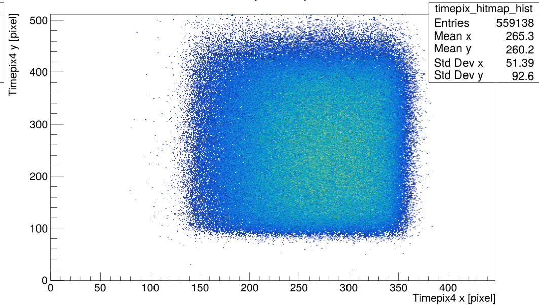
Hitmap Timepix4
