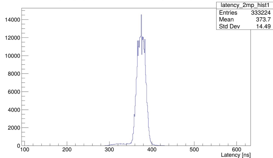
Latency of digital pixel relative cluster with 2 or more pixels x = 6, y = 509, input = 1
