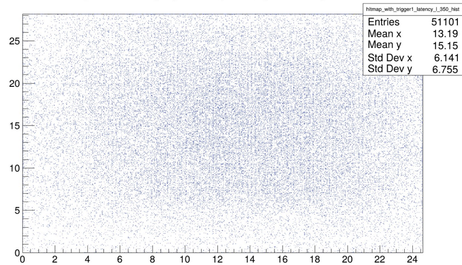
Hitmap. Events with digital pixel x = 6, y = 509, input = 1 latency less than 350
