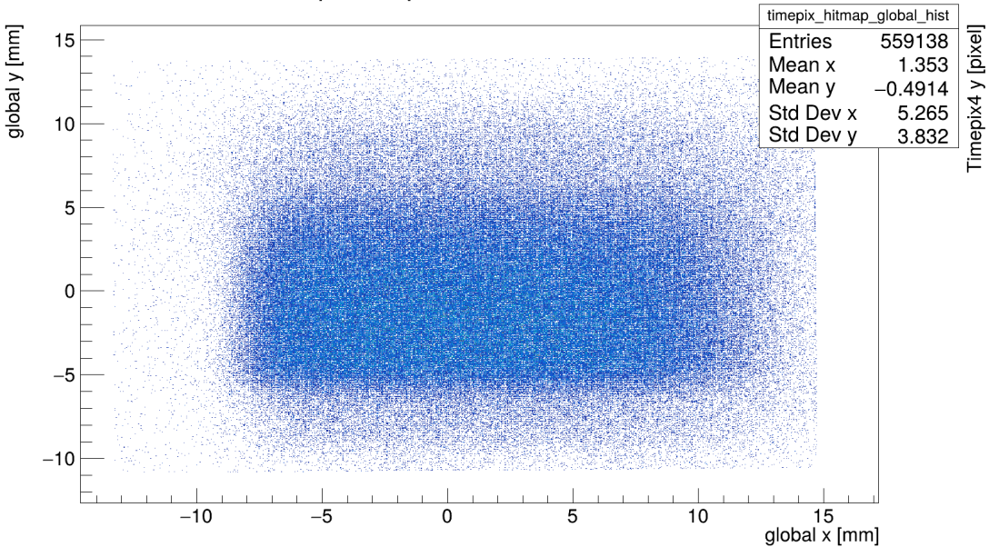
Hitmap Timepix4. Global coordinates
