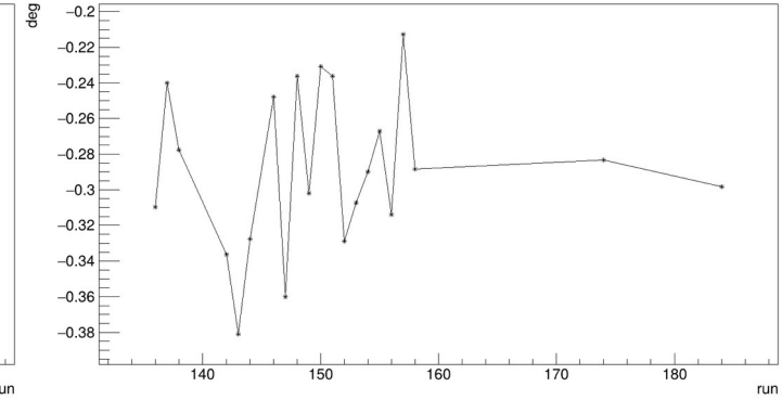
Geometry. Mimosa 1. Rot z
