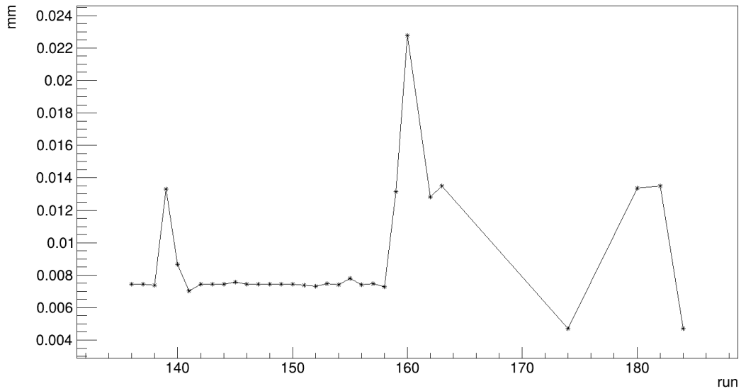
Resolution x. Mimosa 4
