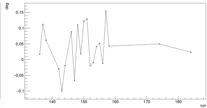
Geometry. Mimosa 0. Rot z
