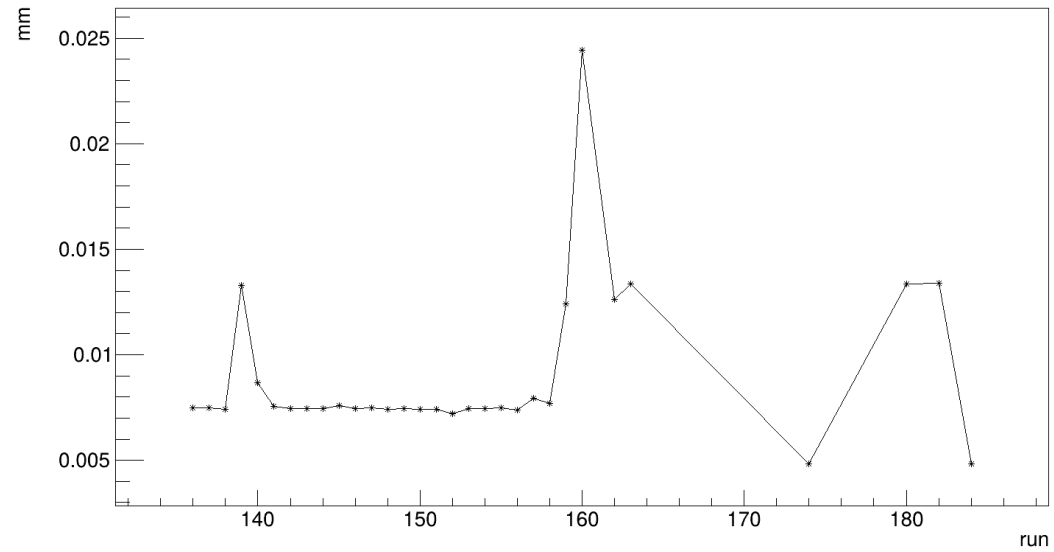
Resolution y. Mimosa 4
