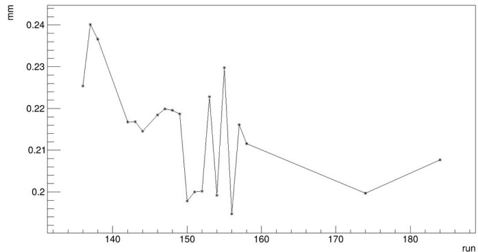
Geometry. Mimosa 1. Shift x
