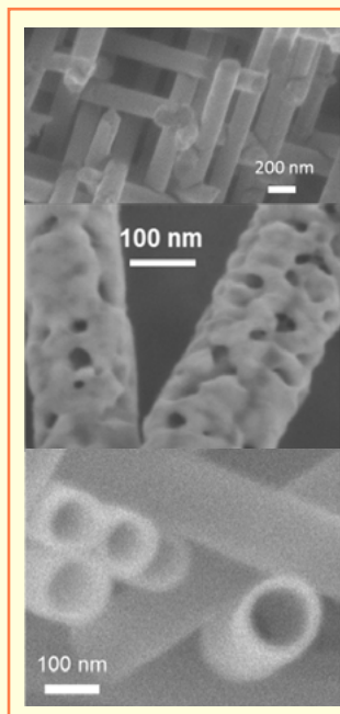
Novel ion-track technology based nanostructures such as nanowire networks (top), porous wires (center) and nanotubes (bottom) with tailored diameter, length and surface.
