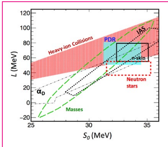
Figure 13. Ranges of strength, S_0 , and slope, L , of the symmetry energy at saturation density, determined from different investigations in nuclear physics and astrophysics.
