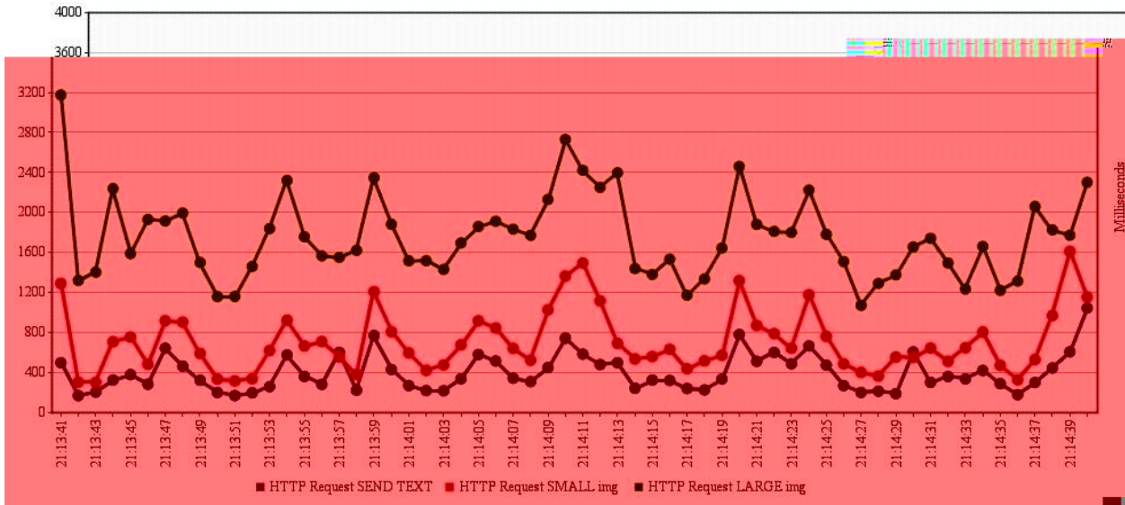
Samples' send-receive average times for different types of requests
