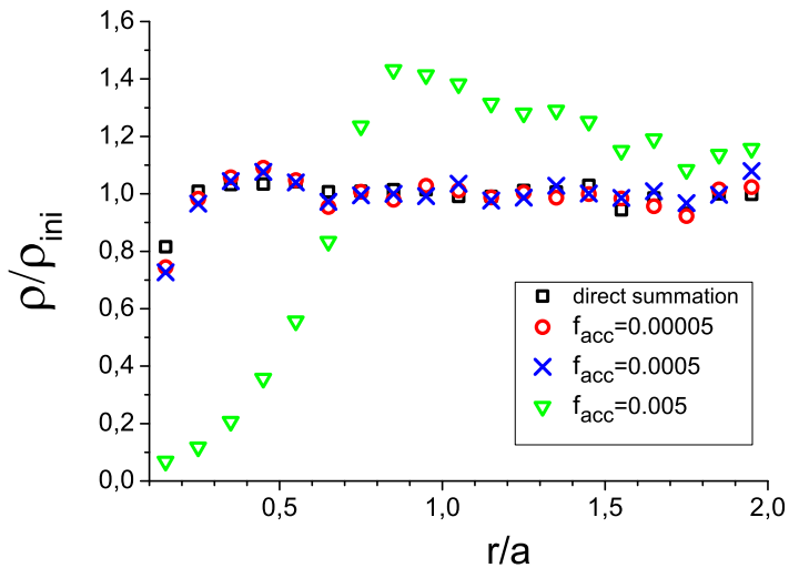
Figure : The density profiles at t = 4.5 \cdot 10^9 years
