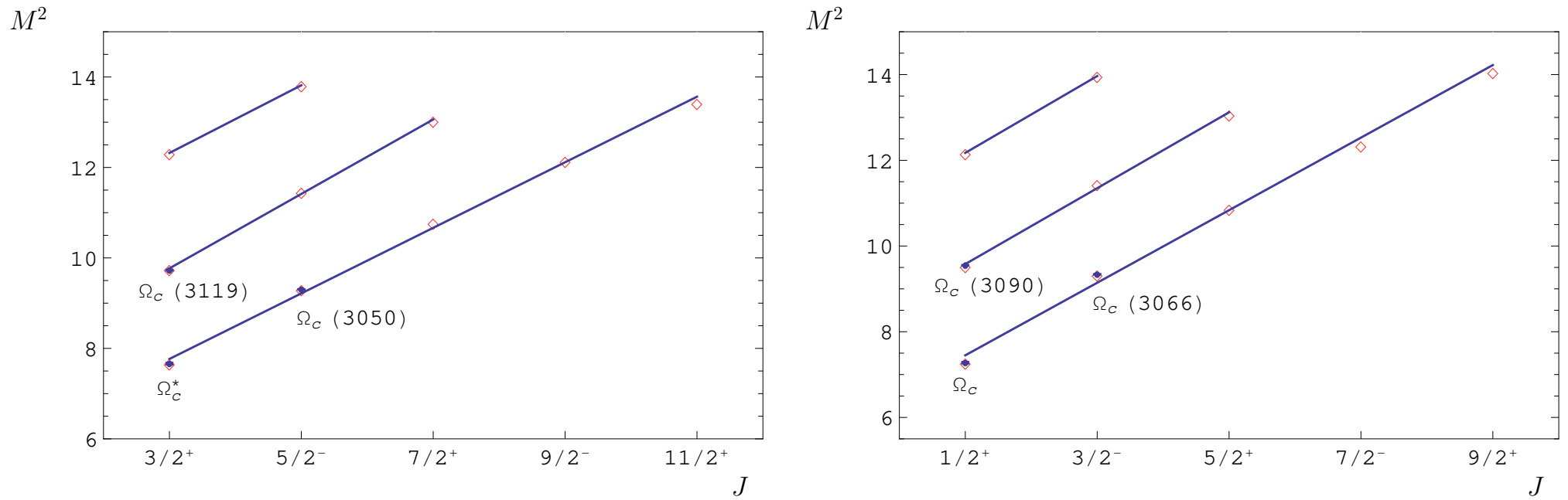
Figure 6: The (J, M^2) Regge trajectories for the \Omega_c baryons. Diamonds are predicted masses. Available experimental data are given by dots with particle names; M^2 is in GeV 2 .
