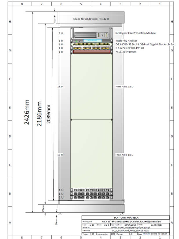
Figure 8; RACK 19" 47 U, Visualization of Standard Equipment.
