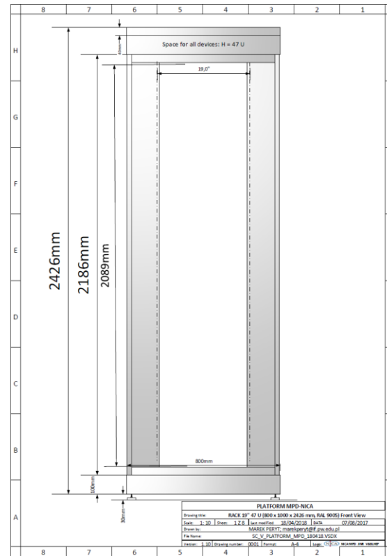
Figure 7; RACK 19" 47 U - Front View, 800 x 1000 x 2426, RAL 9005
