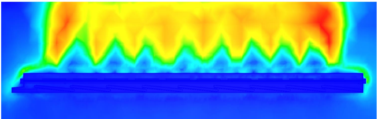
Figure 4 Cross-sections through flow around module of the TOF-MPD
