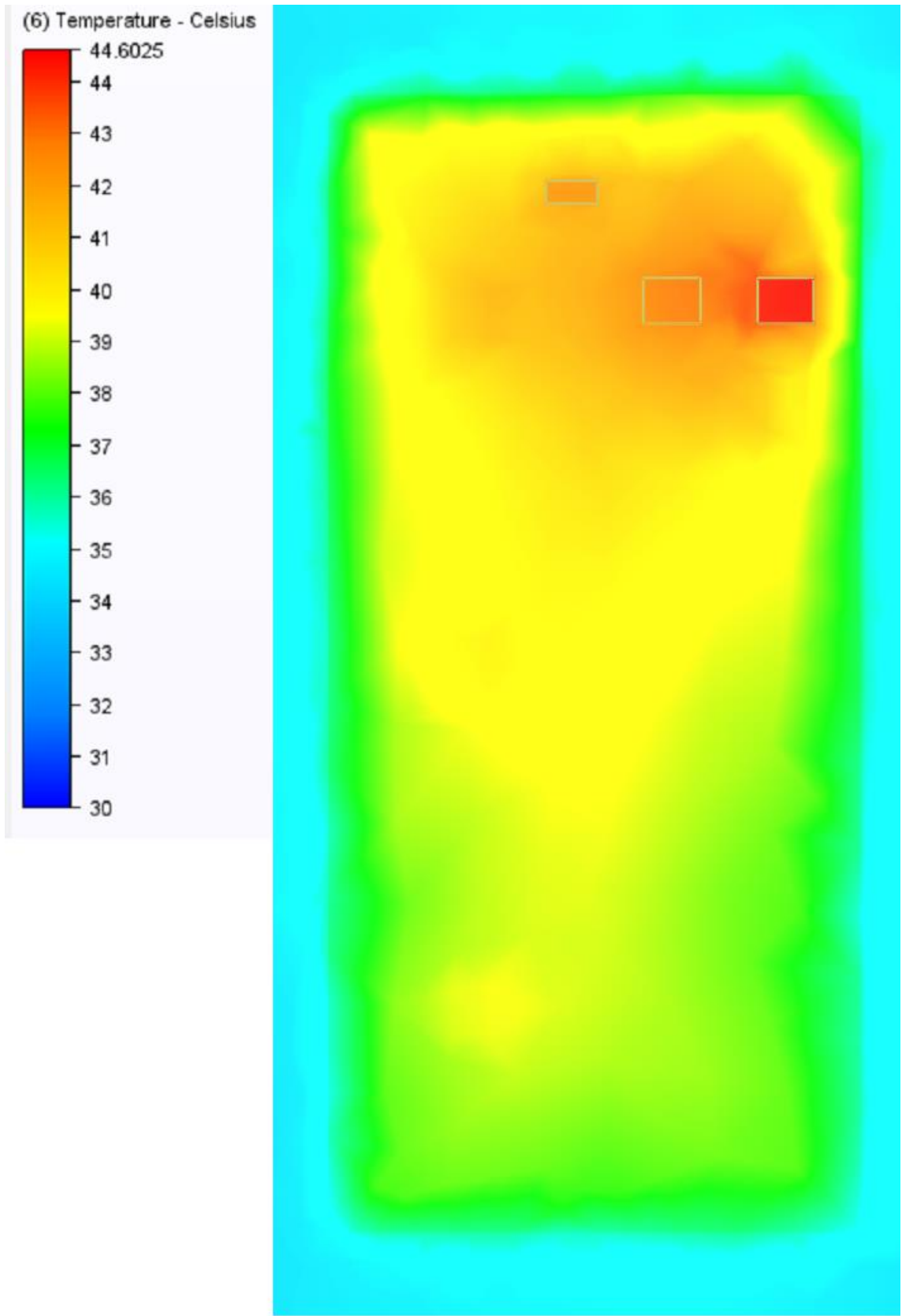
Figure 3 Gradient of temperature on the preamplifiers
